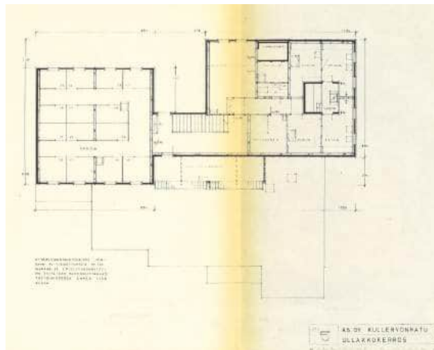
Ullakko krs.
