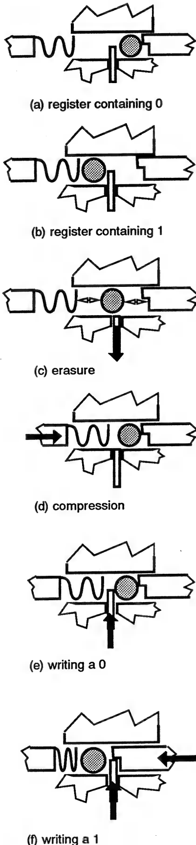
Figure 4 Register operation
