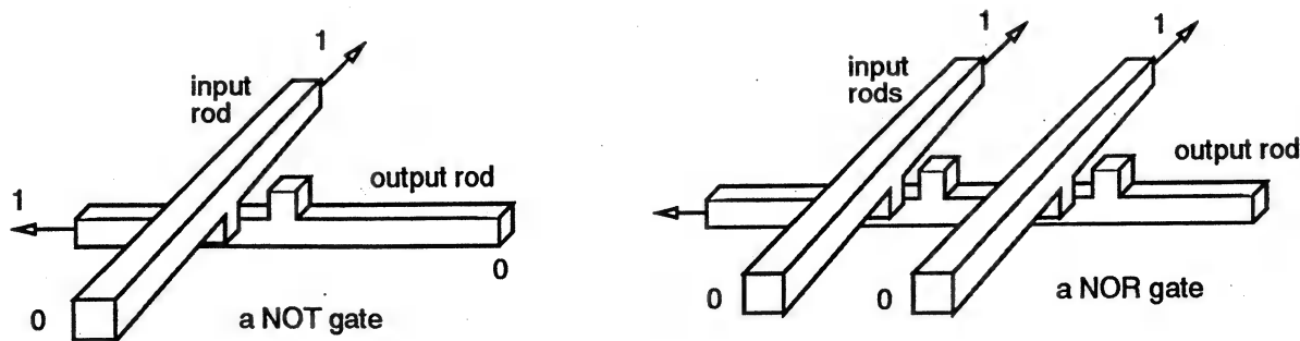
Figure 2. Rod Logic.
