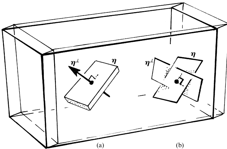
Fig. 18.4 In \mathbb{E}^4 , an r -plane element \eta at a point p has an orthogonal complement \eta^\perp which is a (4 - r) -plane element, where \eta and \eta^\perp never have a direction in common. (a) In particular, if \eta is a 3-plane element, then \eta^\perp is the normal direction to it. (b) If \eta is a 2-plane element, then \eta^\perp is another 2-plane element.
