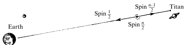
Fig. 29.4 A density matrix can represent a probability mixture of more states than the dimension of the space. In this example: at a point between Earth and Titan, a known initial state of spin \frac{n}{2} (for n > 2 ) splits into a spin \frac{1}{2} particle aimed at Earth and a spin \frac{1}{2}(n-1) particle aimed at Titan. A colleague on Titan measures the latter's spin m -value, and the probability for each of the n possible measurement results is a specific number that can be calculated (at Earth), knowing the initial state, so a specific 2 \times 2 density matrix arises at Earth, composed as a probability mixture of n states. (This clearly also generalizes to a Hilbert space of more than 2 dimensions.)
