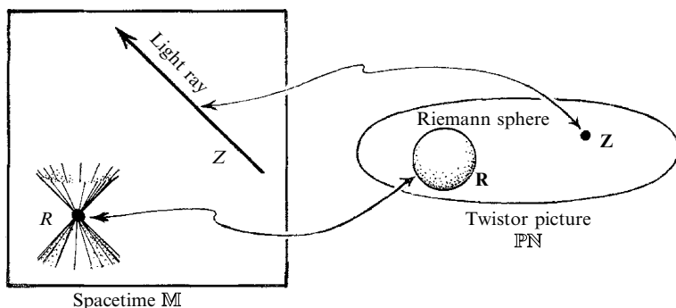
Fig. 33.5 A light ray Z in Minkowski spacetime \mathbb{M} is represented as a single point Z in the twistor space \mathbb{PN} (projective null twistor space); a single point R in \mathbb{M} is represented by a Riemann sphere \mathbf{R} in \mathbb{PN} (this sphere representing the ‘celestial sphere’ of light rays at R ). (For the complete correspondence this requires the compactified Minkowski space \mathbb{M}^\# described in Fig. 33.9.)
