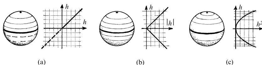
Fig. 10.2 Functions on a sphere S , pictured as sitting in Euclidean 3-space, where h measures the distance above the equatorial plane. (a) The function h itself is smooth on S (negative values indicated by broken lines). (b) The modulus |h| (see Fig. 6.2b) is not smooth along the equator. (c) The square h^2 is smooth all over S .
