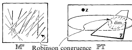
Fig. 33.14 We can obtain a ‘real’ picture of a non-null twistor Z^\alpha by first passing to its complex conjugate \bar{Z}_\alpha , thus defining a complex projective plane in \mathbb{P}^T . This plane is fixed by its intersection with \mathbb{P}\mathbb{N} , which is a 3-real-dimensional locus. This locus defines a 3-parameter family of light rays in \mathbb{M}^\# called a Robinson congruence.
