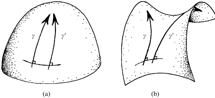
Fig. 14.12 Geodesic deviation when M is a 2-surface (a) of positive (Gaussian) curvature, when the geodesics \gamma, \gamma' bend towards each other, and (b) of negative curvature, when they bend apart.
