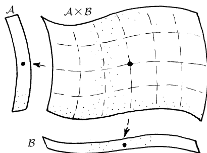
Fig. 31.7 The product manifold \mathcal{A} \times \mathcal{B} (see Fig. 15.3a, §15.2) of two (pseudo-) Riemannian spaces \mathcal{A} and \mathcal{B} is itself (pseudo-)Riemannian. If both \mathcal{A} and \mathcal{B} are Ricci-flat, then so is \mathcal{A} \times \mathcal{B} .
