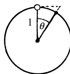
Fig. 18.11 Velocity space in relativity theory is the (unit) hyperbolic space \mathcal{H}^+ , where the rapidity \rho (= \tanh^{-1} v) measures hyperbolic distance along \mathcal{H}^+ (the speed of light c = 1 corresponding to infinite \rho ). This is analogous (by ‘signature flip’) to distance along a unit circle being the angle \theta subtended at its centre.
