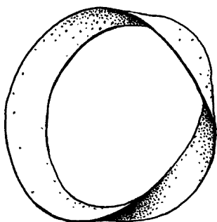
Fig. 12.15 The Möbius strip: an example of a non-orientable space.
