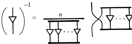
Fig. 13.7 The inverse T^{-1} of a non-singular (n \times n) matrix T given here explicitly in diagrammatic form, using the diagrammatic form of the Levi-Civita antisymmetric quantities \varepsilon_{a\dots c} and \varepsilon^{a\dots c} (normalized by \varepsilon_{a\dots c} \varepsilon^{a\dots c} = n! ) introduced in §12.7 and depicted in Fig. 12.18.
