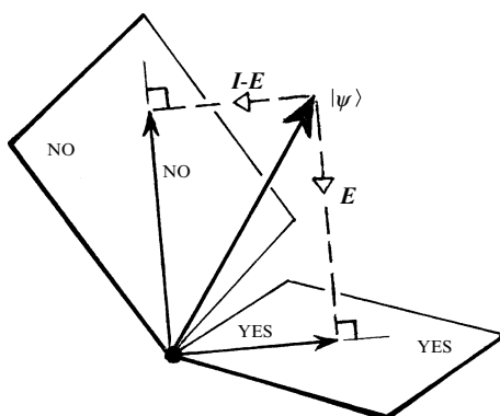
Fig. 22.4 The geometric nature, within \mathbf{H} , of the projection postulate. The eigenspaces of the projector \mathbf{E} are indicated, the horizontal plane representing the eigenvalue 1 (YES) and the vertical plane, the eigenvalue 0 (NO). The picture illustrates the decomposition |\psi\rangle = \mathbf{E}|\psi\rangle + (\mathbf{I} - \mathbf{E})|\psi\rangle of |\psi\rangle into two orthogonal parts, where \mathbf{E}|\psi\rangle is the projection of |\psi\rangle to within the YES space (the result of the measurement yielding YES) and (\mathbf{I} - \mathbf{E})|\psi\rangle , the projection to within the NO space (from the result NO). The probability in each case is given by the exact proportionality factor whereby the squared (Hermitian) length \|\psi\|^2 of |\psi\rangle is reduced in the projection (state vectors not normalized).
