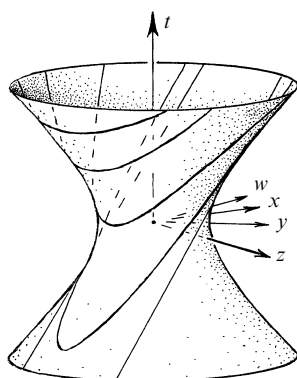
Fig. 28.7 The de Sitter spacetime (pictured as a hyperboloid, with two spatial dimensions suppressed) is a Lorentzian ‘4-sphere’ (of imaginary radius, giving intrinsic metric signature +- - - ) in Minkowski 5-space \mathbb{M}^5 (whose metric is ds^2 = dt^2 - dw^2 - dx^2 - dy^2 - dz^2 ). To get the steady-state model, we ‘cut’ the hyperboloid into half, along t = w ; constant time being given by constant positive t - w .
