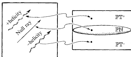
Fig. 33.6 The real 5-manifold \mathbb{IPN} divides projective twistor space \mathbb{IP}^3 into two complex-3-manifold pieces \mathbb{IP}^{3+} and \mathbb{IP}^{3-} , these representing massless particles of positive and of negative helicity, respectively.
