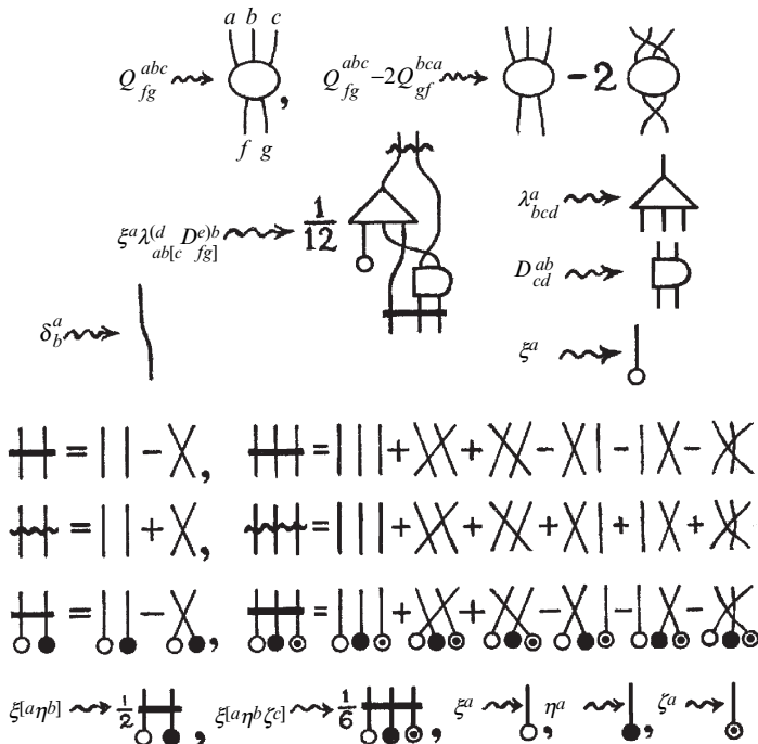
Fig. 12.17 Diagrammatic tensor notation. The [^3_2] -valent tensor Q is represented by an oval with 3 arms and 2 legs, where the general [^p_q] -valent tensor picture would have p arms and q legs. In an expression such as Q_{fg}^{abc} - 2Q_{gf}^{bca} , the diagrammatic notation uses positioning on the page of the ends of the arms and legs to keep track of which index is which, instead of employing individual index letters. Contractions of tensor indices are represented by the joining of an arm and a leg, as illustrated in the diagram for \xi^a \lambda_{ab[c} D^e]^{b}_{fg}] . This diagram also illustrates the use of a thick bar across index lines to denote antisymmetrization and a wiggly bar to represent symmetrization. The factor \frac{1}{12} in the diagram results from the fact that (to facilitate calculations) the normal factorial denominator for symmetrizers and antisymmetrizers is omitted in the diagrammatic notation (so here we need \frac{1}{2!} \times \frac{1}{3!} = \frac{1}{12} ). In the lower half of the diagram, antisymmetrizers and symmetrizers are written out as ‘disembodied’ expressions (by use of the diagrammatic representation of the Kronecker delta \delta^a_b that will be introduced in §13.3, Fig. 13.6c). This is then used to express the (multivector) wedge products \xi \wedge \eta and \xi \wedge \eta \wedge \zeta .
