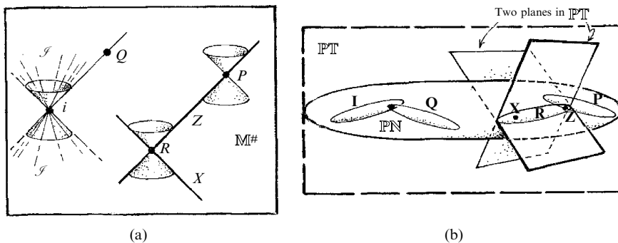
Fig. 33.12 The geometry of the basic loci in \mathbb{M}^\# and \mathbb{P}^3\mathbb{N} , given by the incidence relation of the twistor correspondence. (a) Fix a point (projective null twistor) \mathbf{Z} in \mathbb{P}^3\mathbb{N} . The points of \mathbb{M}^\# (e.g. P, R ) which are incident with \mathbf{Z} constitute a light ray, since all such points are null separated from one another. (b) Fix a point R in \mathbb{M}^\# . The points of \mathbb{P}^3\mathbb{N} (e.g. \mathbf{Z}, \mathbf{X} ) that are incident with R (lying on the intersection of two complex planes in \mathbb{P}^3\mathbb{T} ) constitute a complex projective line, which is a Riemann sphere. Points P and R in \mathbb{M}^\# which are null separated along the light ray \mathbf{Z} have corresponding Riemann spheres \mathbf{P} and \mathbf{R} , which intersect in the single point \mathbf{Z} . (I have drawn these Riemann spheres very elongated, as a compromise with the fact that they are also projective straight lines in the projective geometry of \mathbb{P}^3\mathbb{T} !) A particular one of these Riemann spheres is \mathbf{I} , which represents the point i in \mathbb{M}^\# . The point i specifies spacelike/timelike infinity; it is the vertex of the light cone \mathcal{S} at infinity. Any other point Q of \mathcal{S} is represented in \mathbb{P}^3\mathbb{N} , by a projective line \mathbf{Q} meeting \mathbf{I} .
