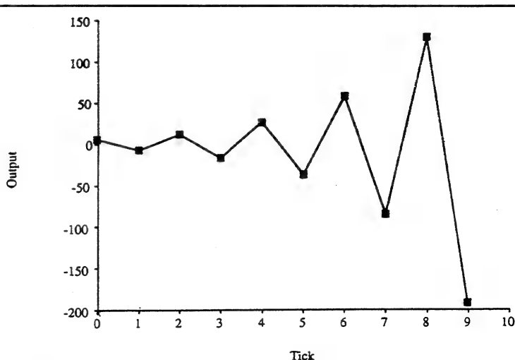
Figure 5. Output of the network in Figure 1, with no input, w_2 = -1.5 , initial output = 5
