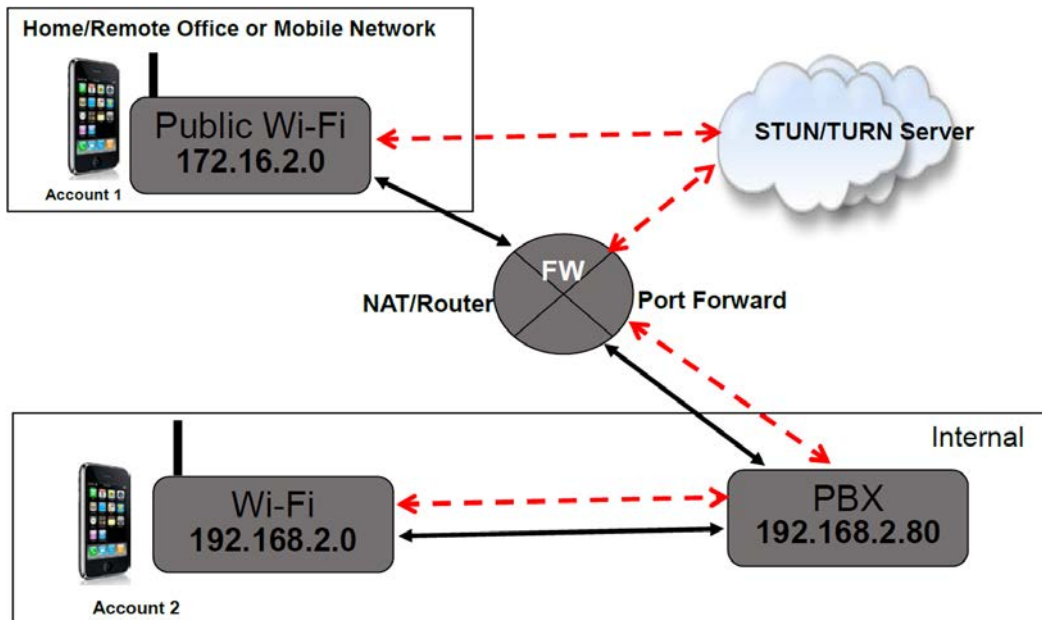
Figure 2-90 Without a Registered Public Domain
