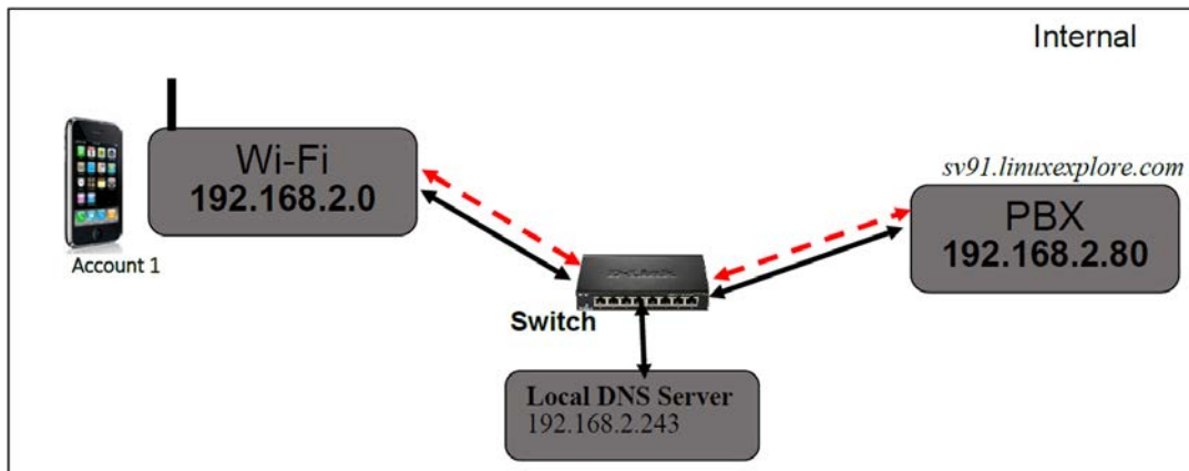
Figure 2-89 Example of MLC on Local Network
