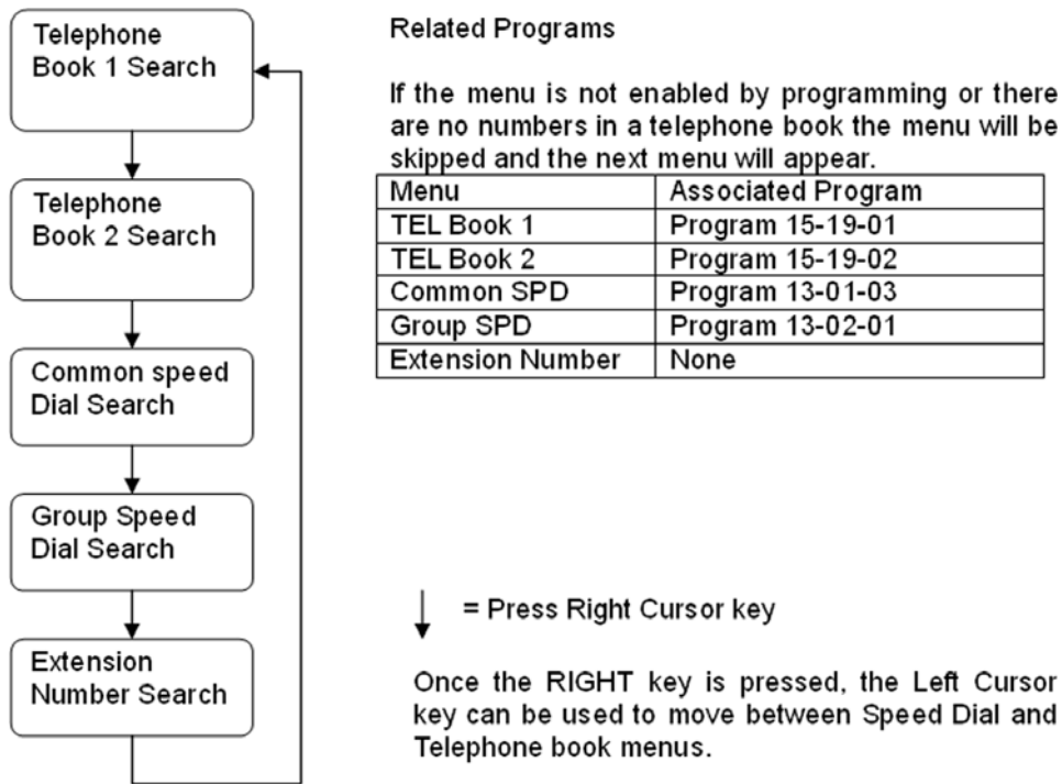
Figure 2-154 Right Cursor Key Operation Flow Chart
