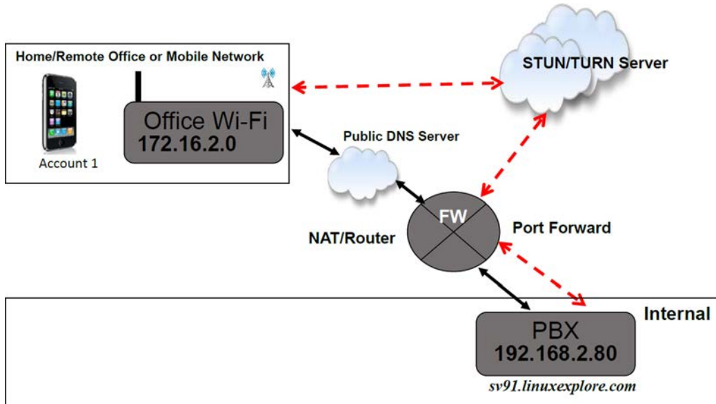
Figure 2-88 Example of MLC on Public Network
