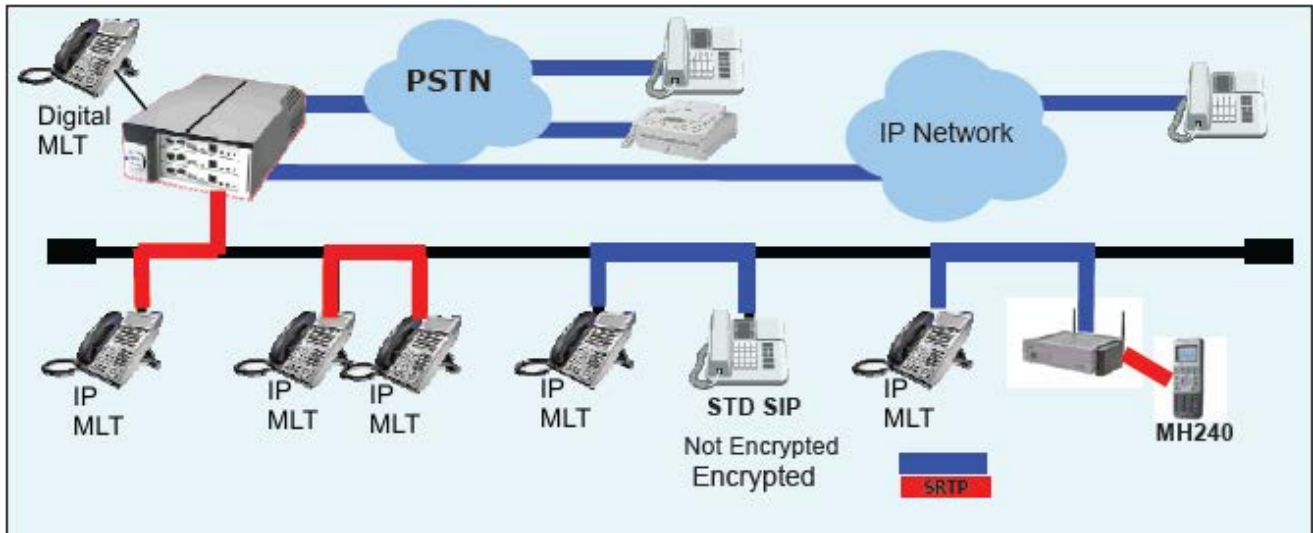
Figure 2-165 SV9100 Encryption Configuration
