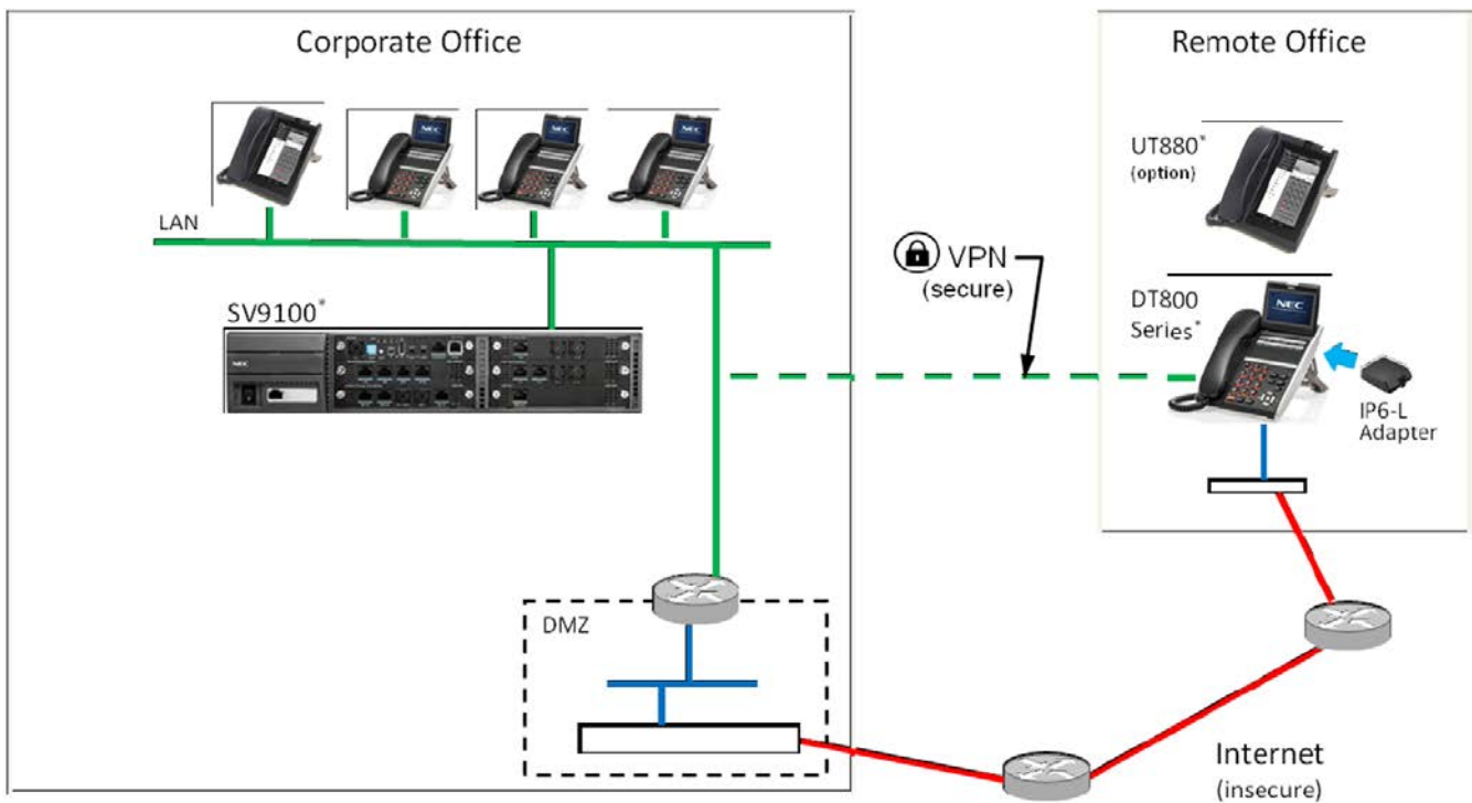
Figure 2-83 Example of InVPN Configuration
