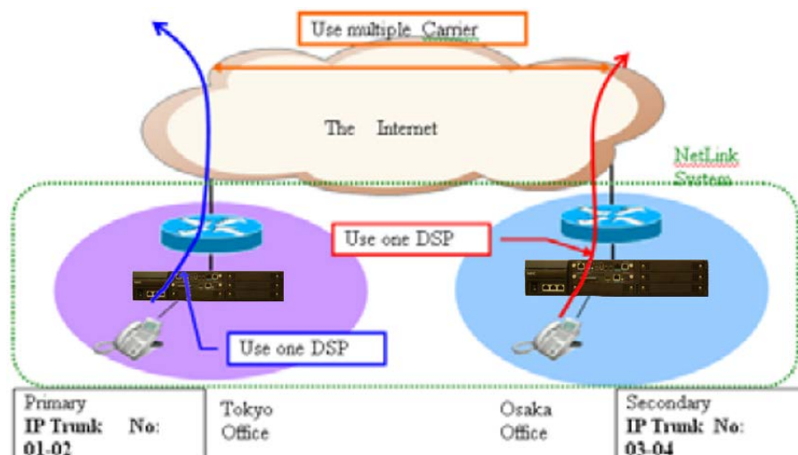
Figure 2-164 Example – NetLink Multiple Carrier
