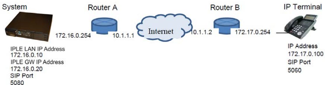
Figure 2-84 Example – NAT Traversal
