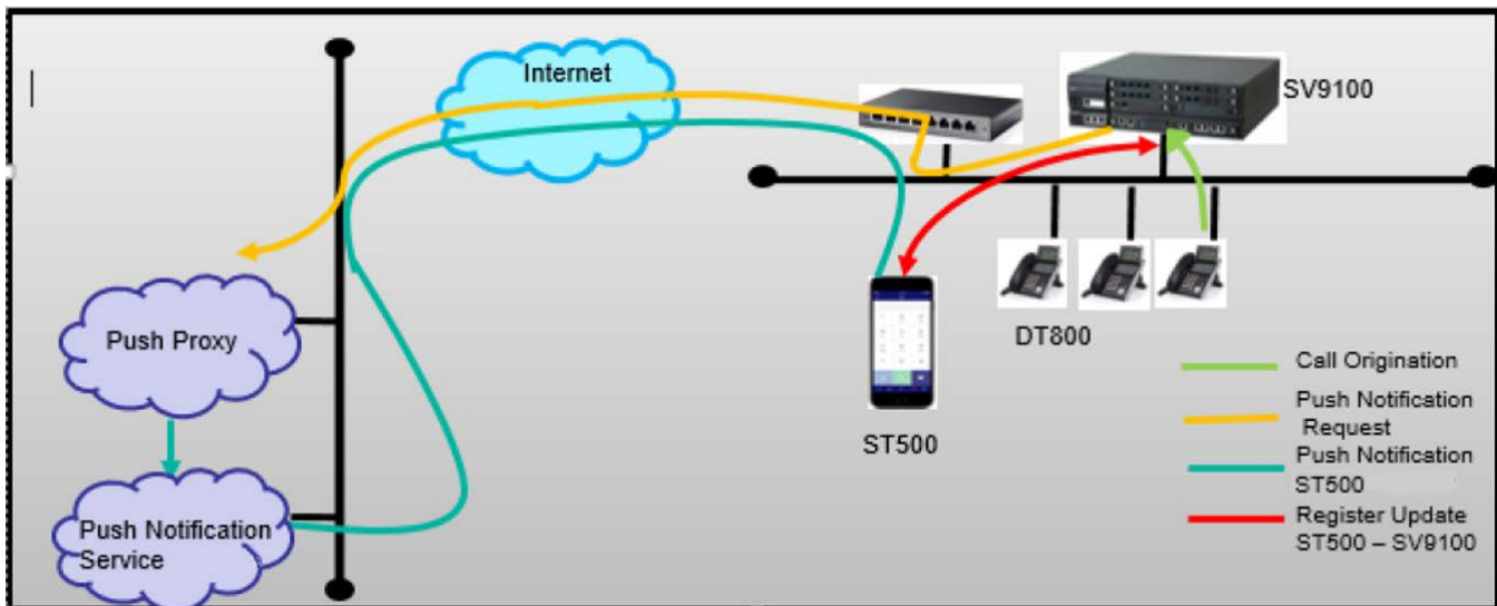
Figure 2-107 Example of Push Notification
