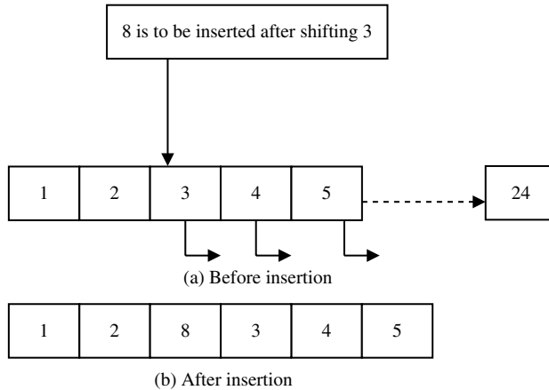
Figure 7.12 Insertion of element
