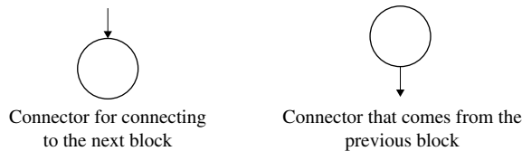
Figure 1.22 Connector symbol
