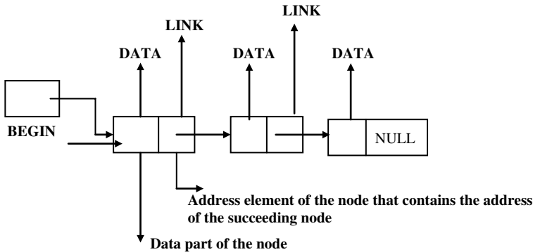
Figure 16.9 Linked list
