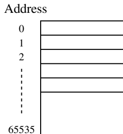
Figure 9.2 Memory address
