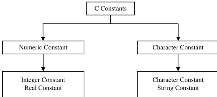
Figure 2.4 C constants
