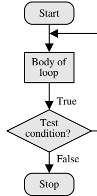
Figure 6.2 The do-while statement
