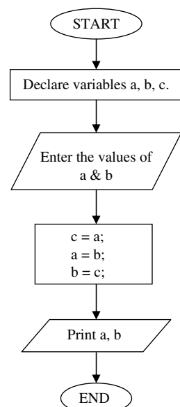
Flowchart for swapping two numbers:
