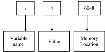
Figure 7.1 Variable mechanisms
