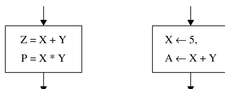
Figure 1.23 Process symbol
