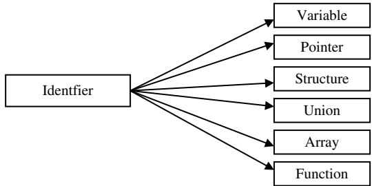
Figure 2.3 Identifiers
