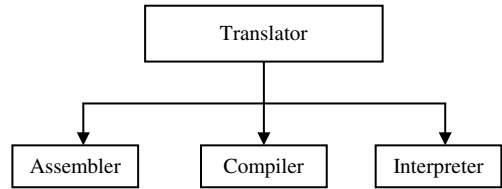
Figure 1.8 Translators
