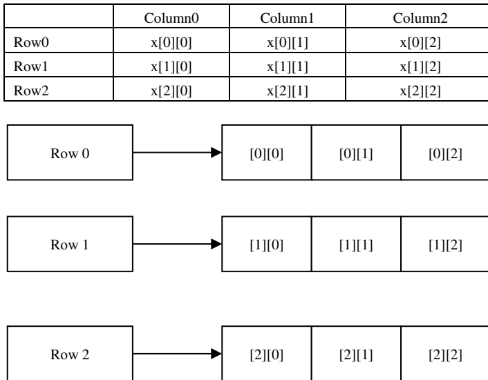
Figure 7.10 Two-dimensional array
