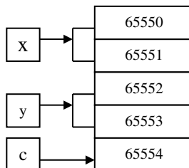
Figure 9.3 Memory allocated
