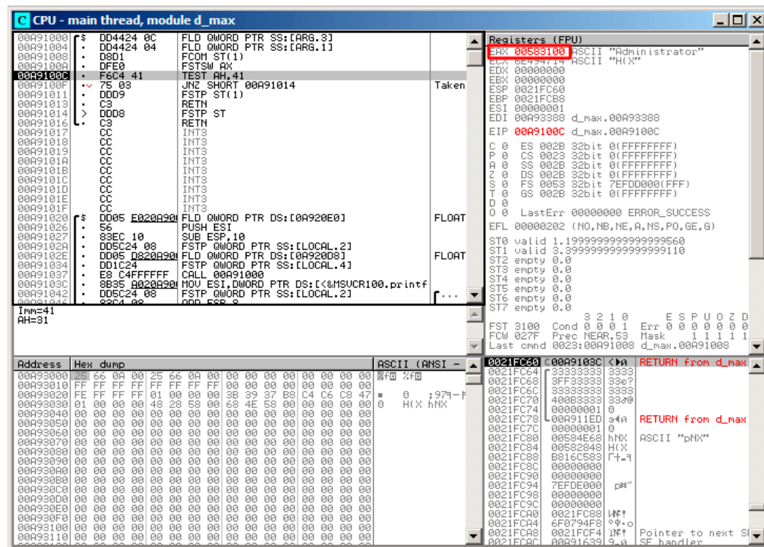
Figure 1.79: OllyDbg: FNSTSW is executed
