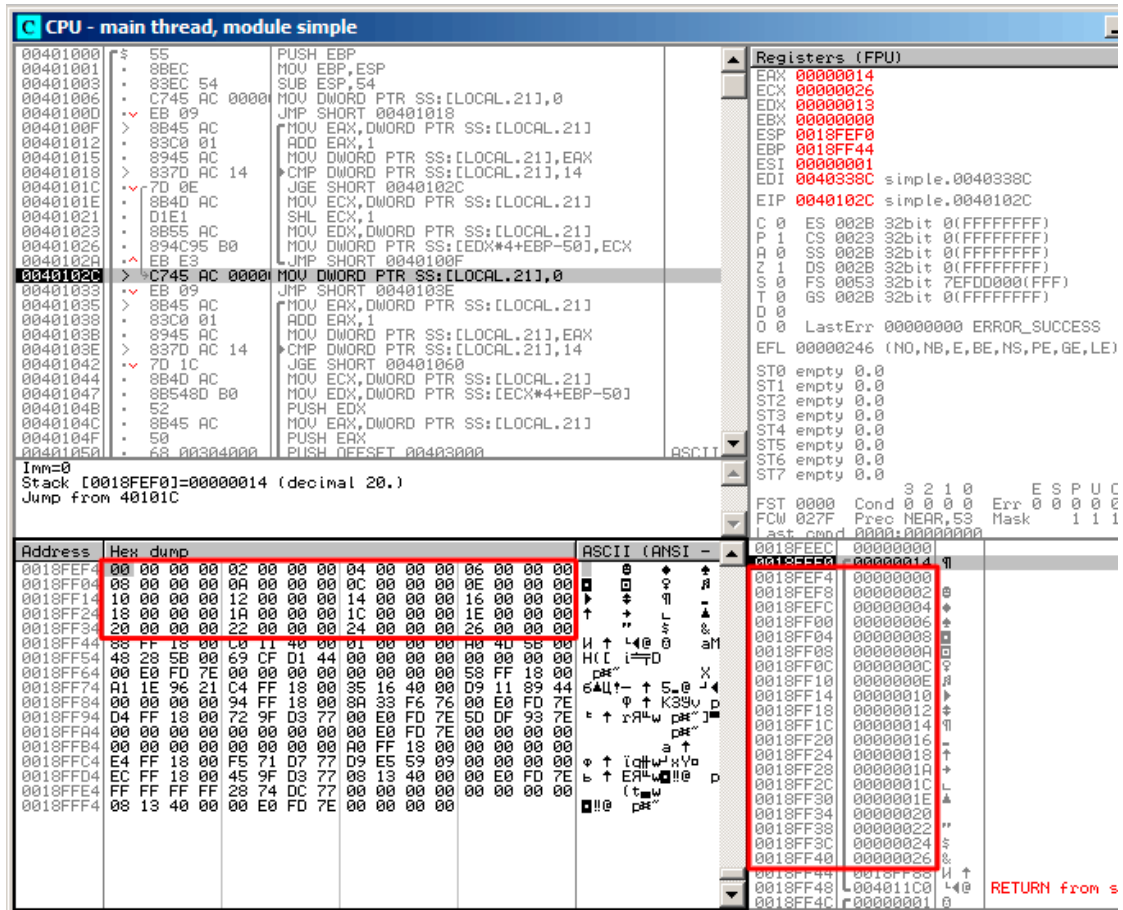
Figure 1.87: OllyDbg: after array filling
