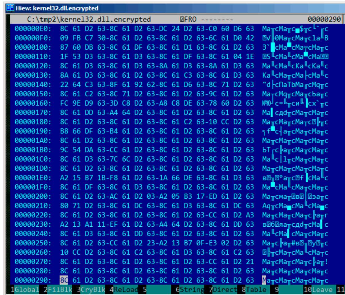
Figure 9.7: “Encrypted” PE-header
