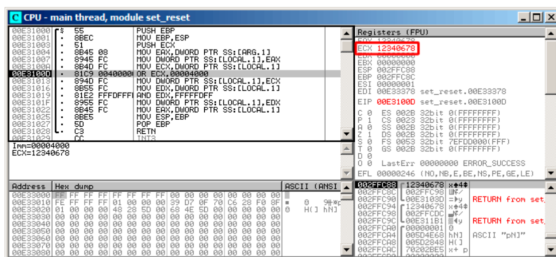
Figure 1.94: OllyDbg: value is loaded into ECX
