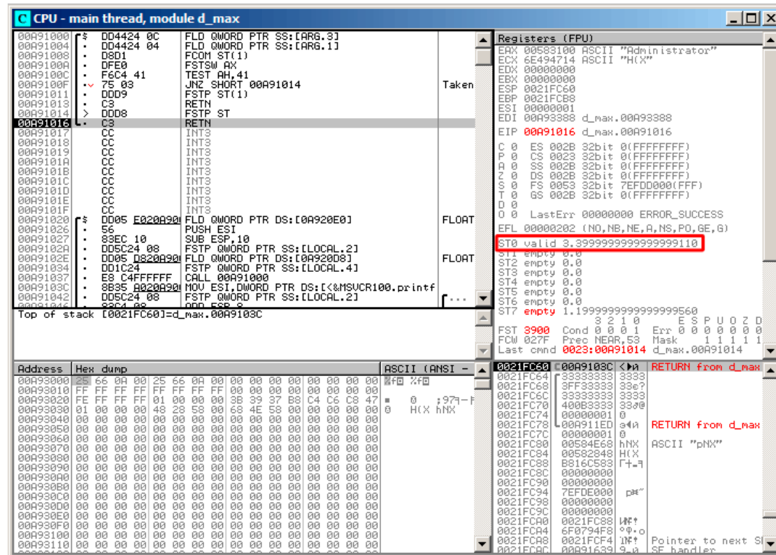
Figure 1.81: OllyDbg: FSTP is executed
