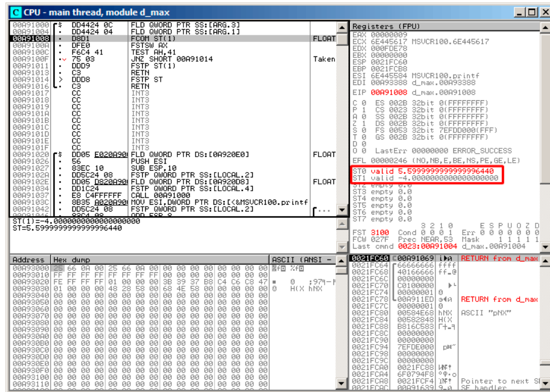
Figure 1.82: OllyDbg: both FLD are executed
