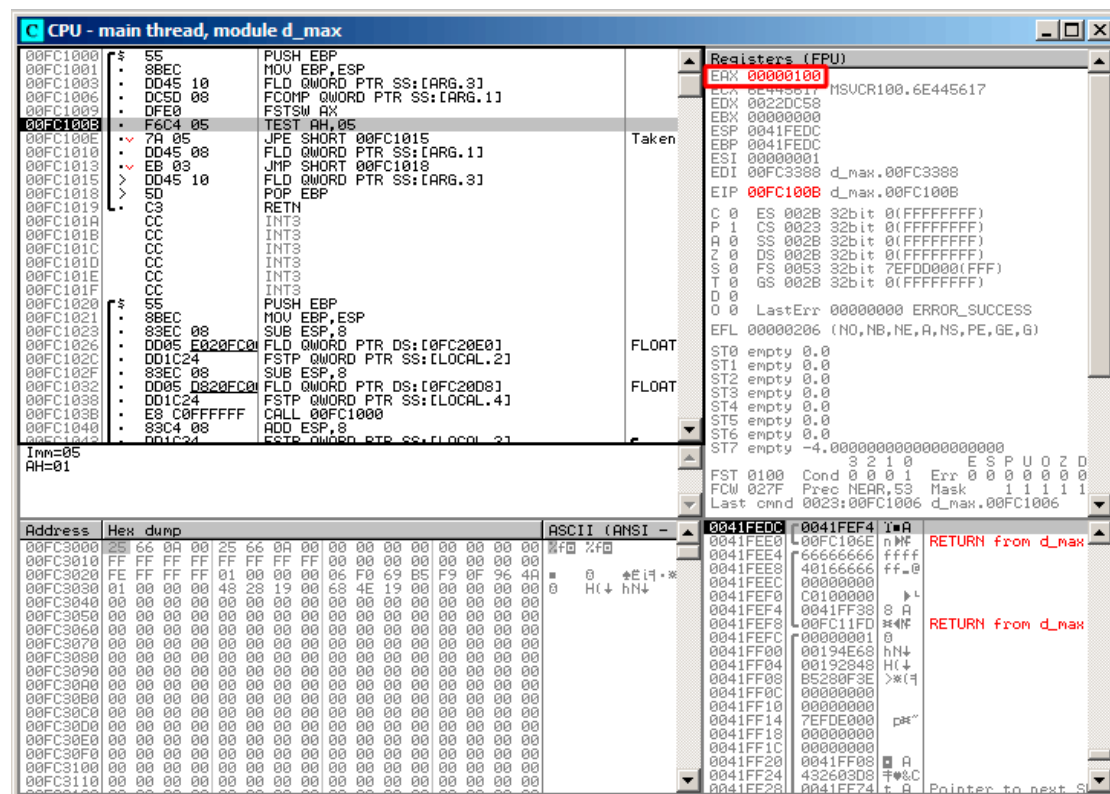
Figure 1.74: OllyDbg: FNSTSW executed
