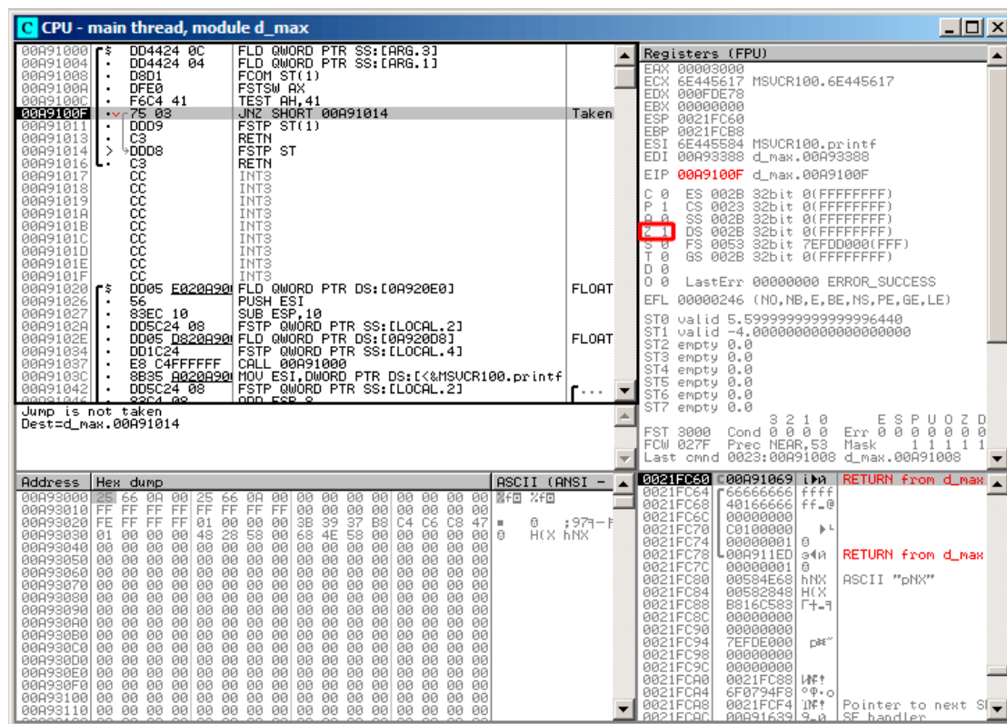
Figure 1.85: OllyDbg: TEST has been executed
