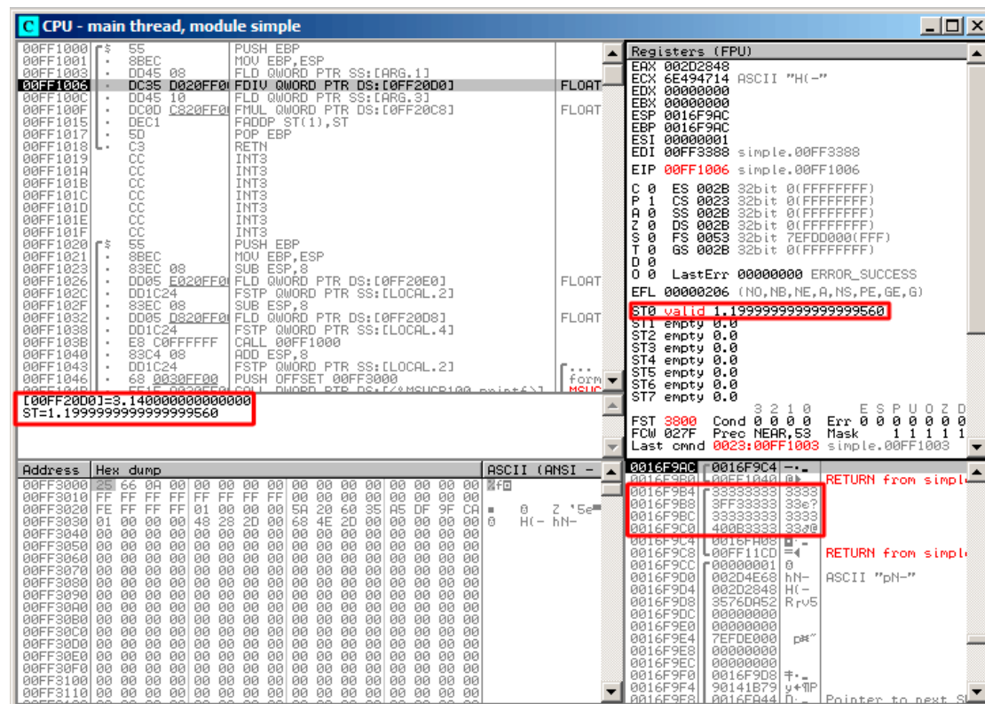
Figure 1.62: OllyDbg: the first FLD has been executed
