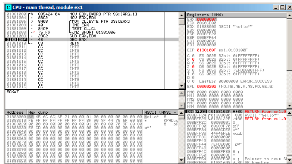
Figure 1.61: OllyDbg: EAX to be decremented now
