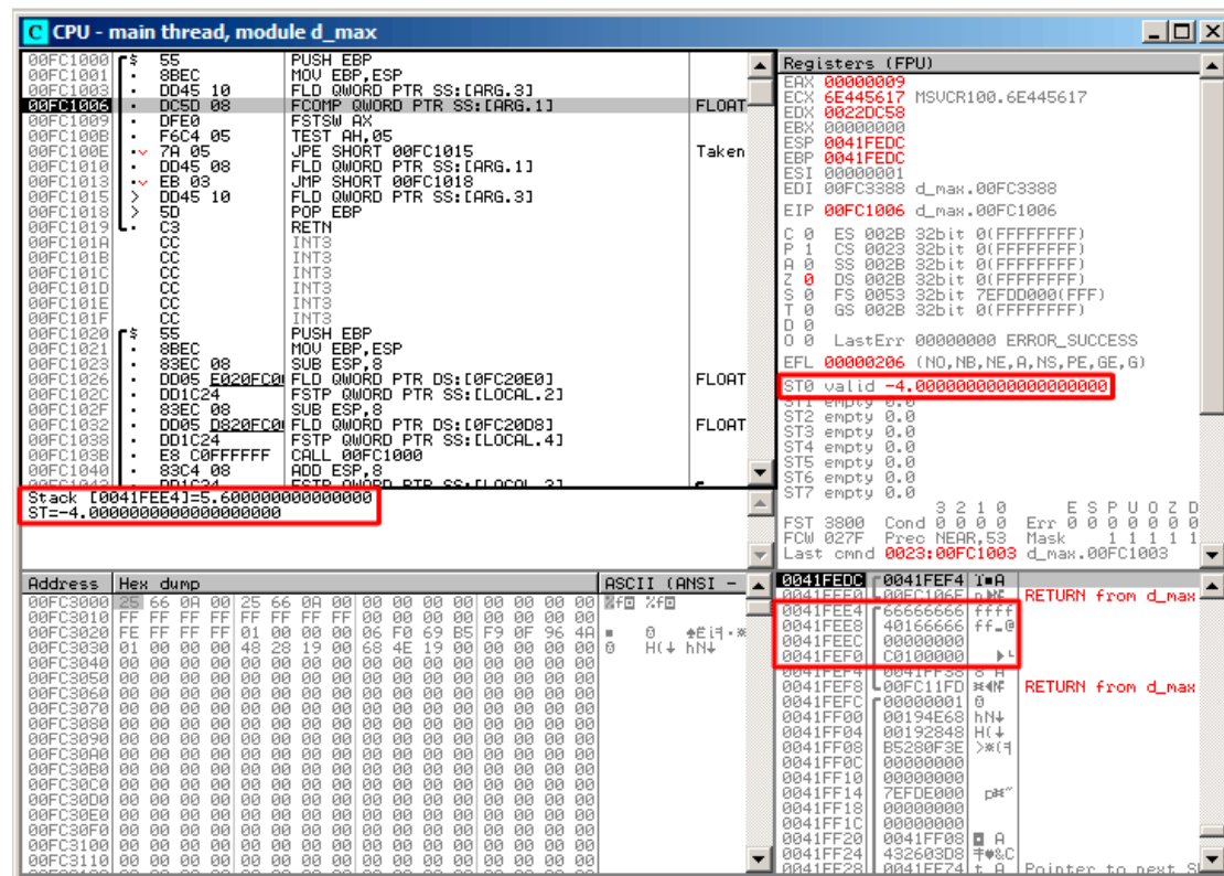
Figure 1.72: OllyDbg: first FLD executed
