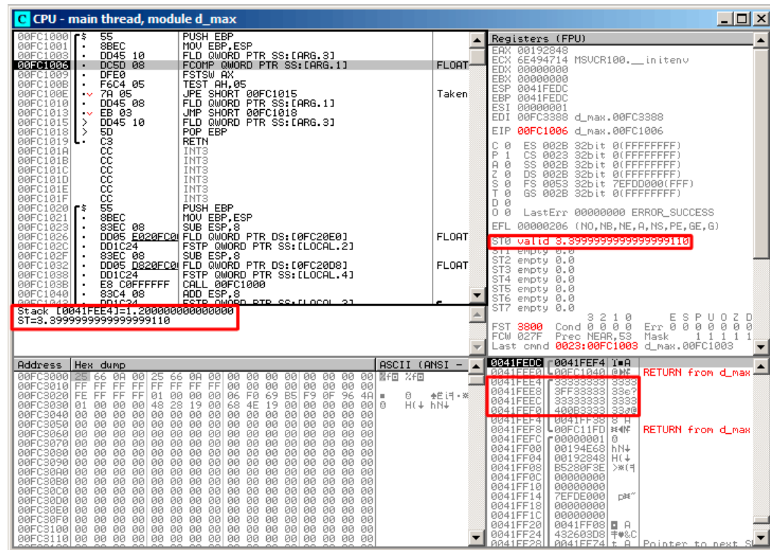
Figure 1.67: OllyDbg: first FLD has been executed
