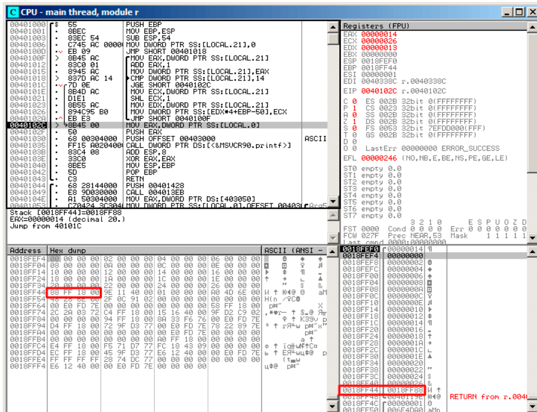
Figure 1.88: OllyDbg: reading of the 20th element and execution of printf()
