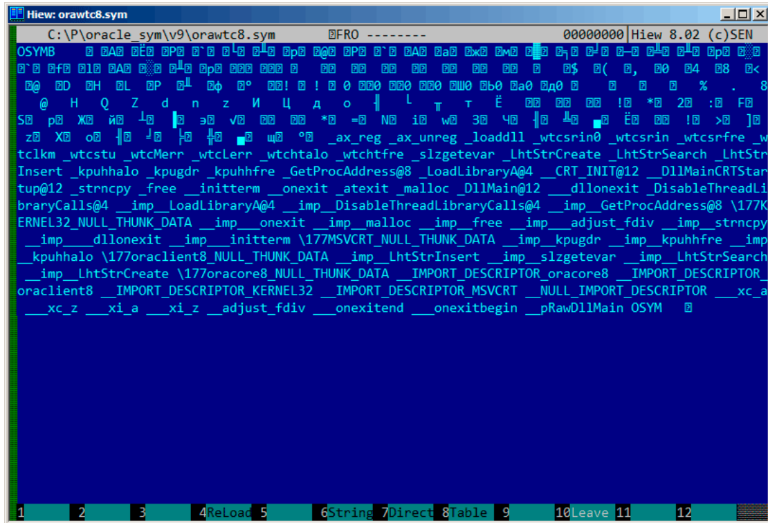
Figure 9.22: The whole file in Hiew
