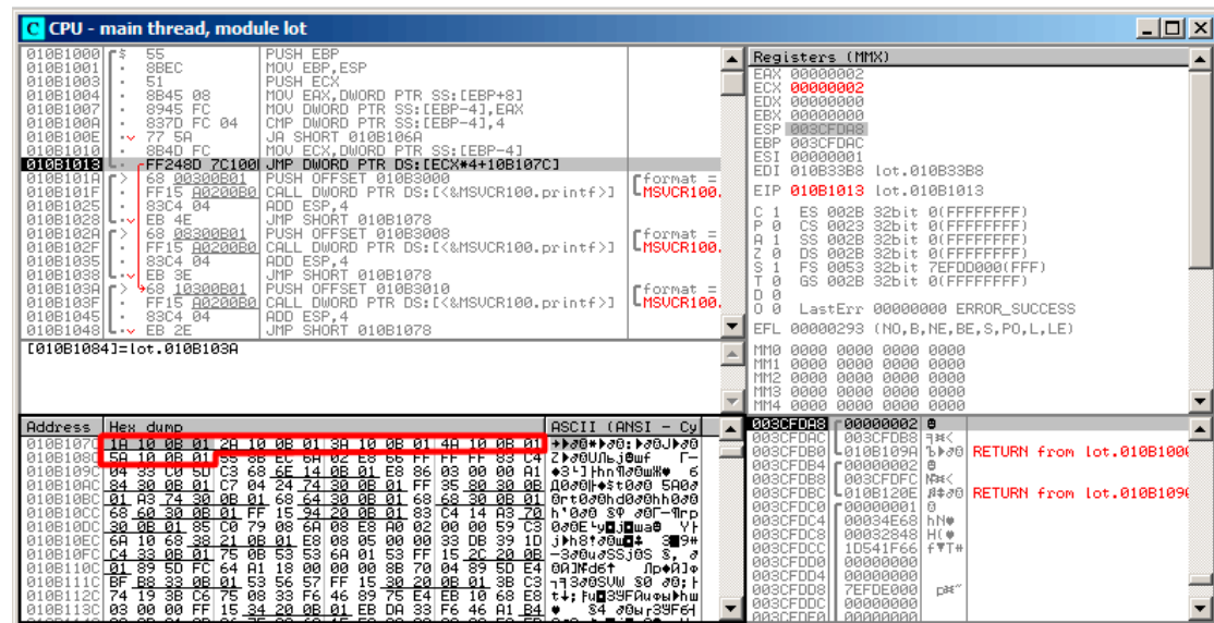
Figure 1.52: OllyDbg: calculating destination address using jumptable
