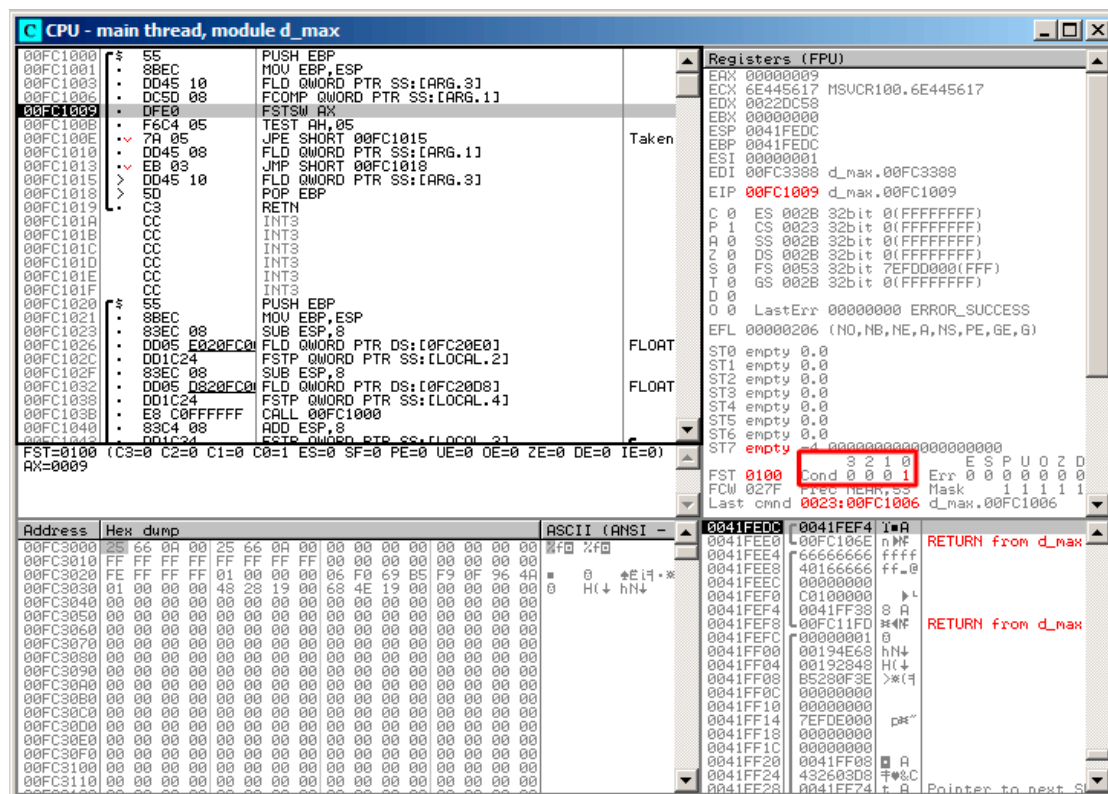
Figure 1.73: OllyDbg: FCOMP executed
