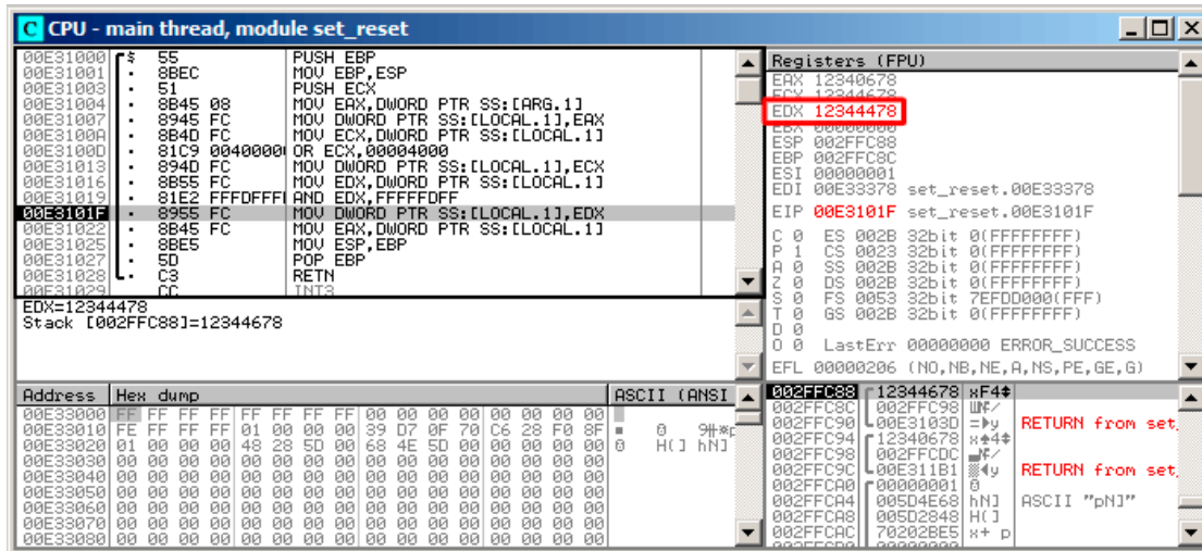
Figure 1.97: OllyDbg: AND executed
