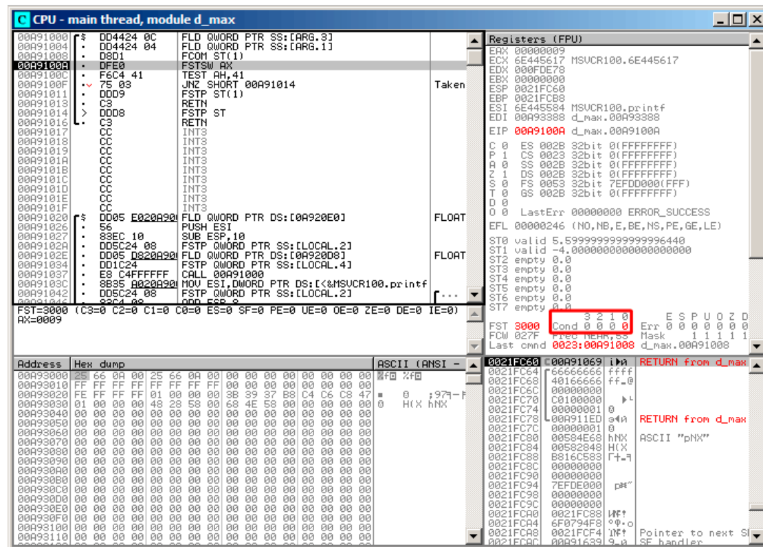
Figure 1.83: OllyDbg: FCOM is finished
