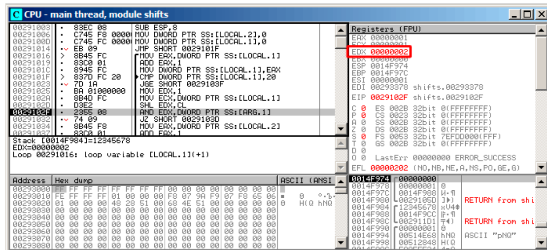
Figure 1.99: OllyDbg: i = 1 , EDX = 1 \ll 1 = 2
