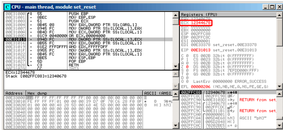
Figure 1.95: OllyDbg: 0R executed
