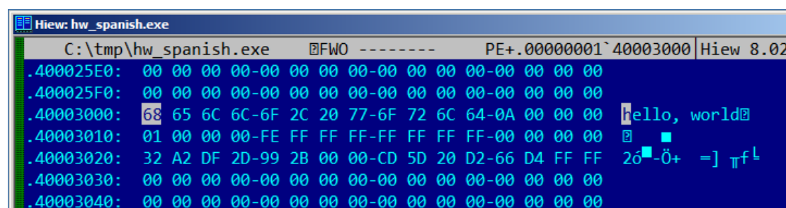
Figure 1.1: Hiew
