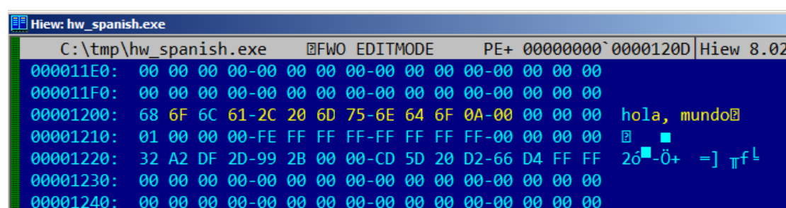
Figure 1.2: Hiew
