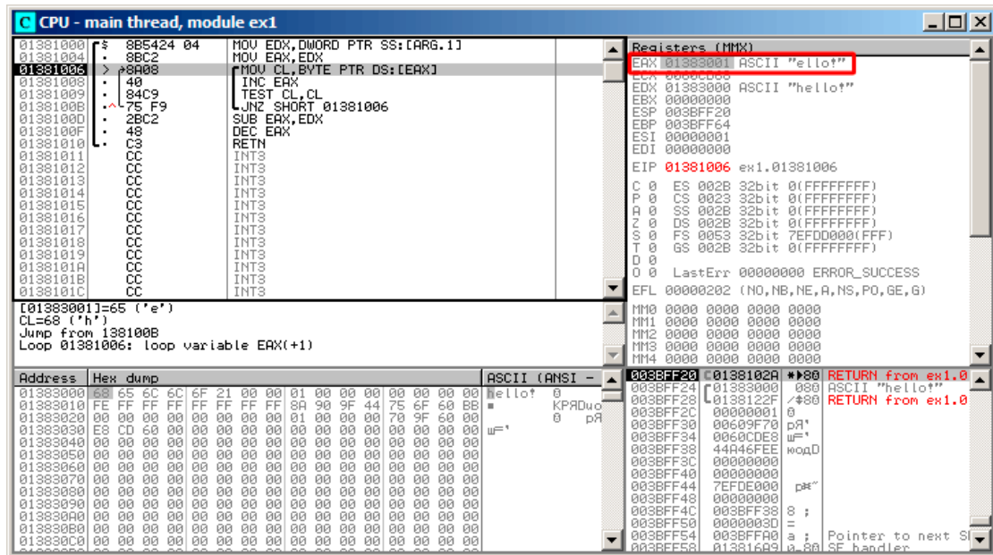
Figure 1.59: OllyDbg: second iteration start
