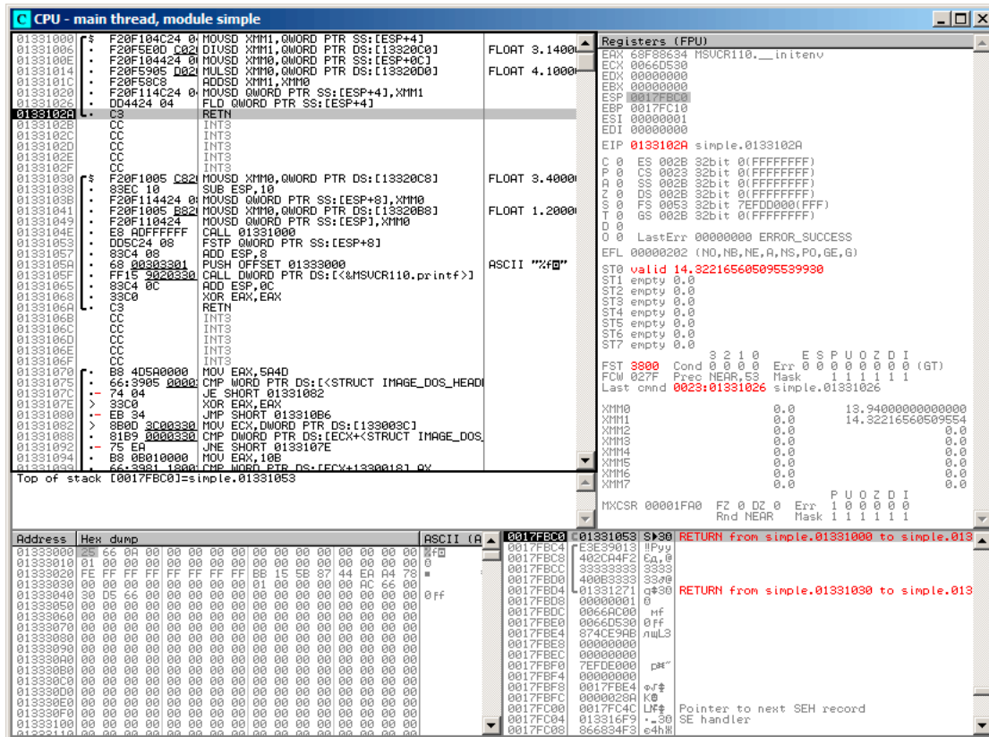
Figure 1.117: OllyDbg: FLD left function result in ST(0)
