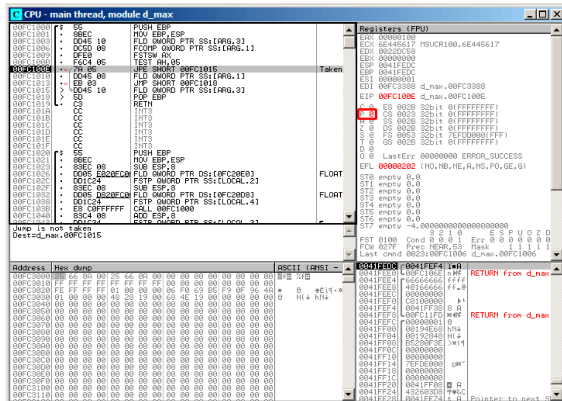
Figure 1.75: OllyDbg: TEST executed
