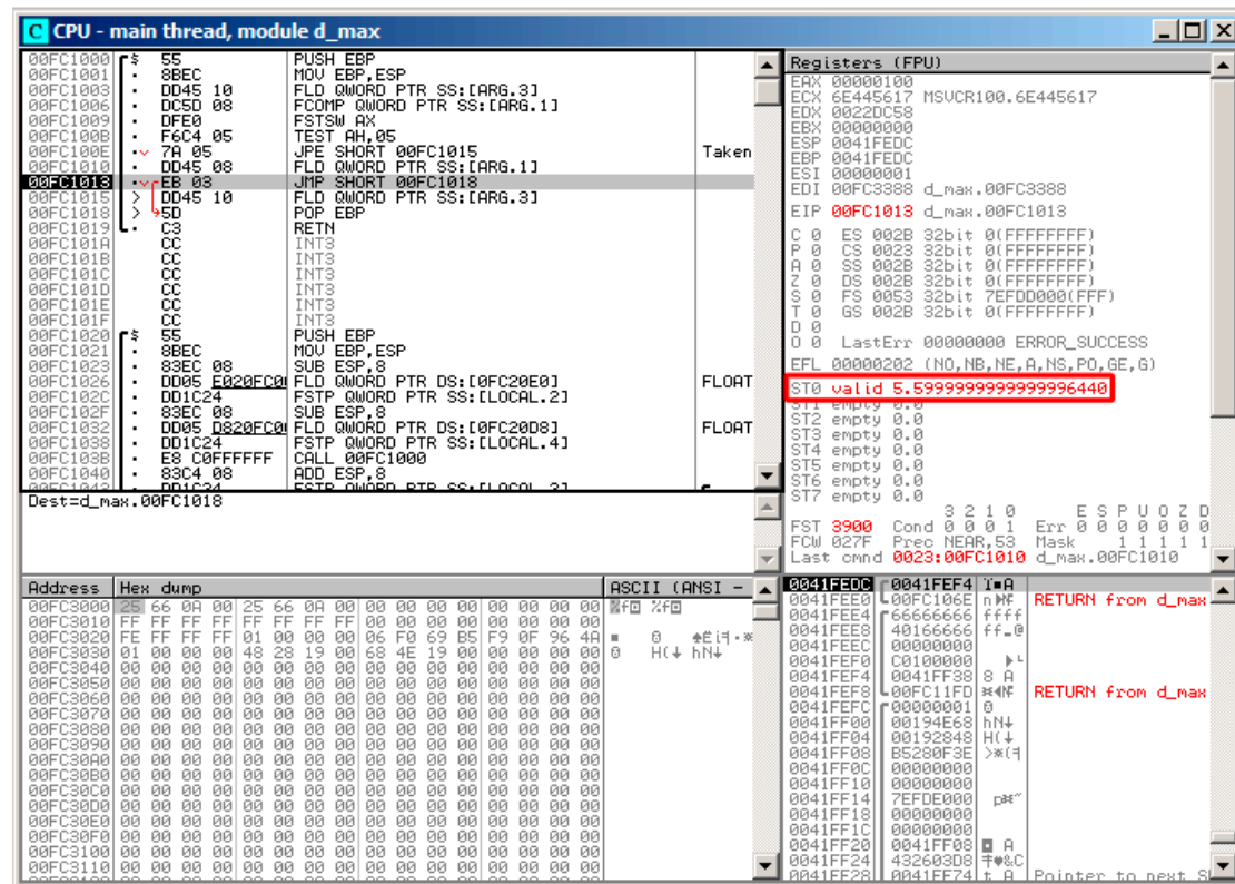
Figure 1.76: OllyDbg: second FLD executed
