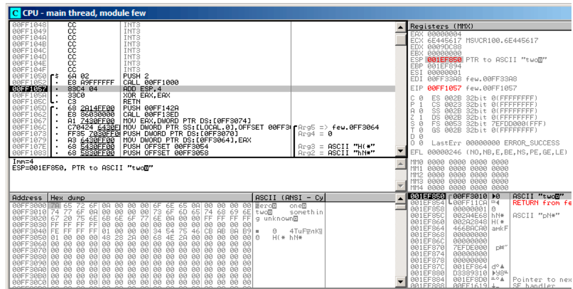
Figure 1.49: OllyDbg: return to main()
