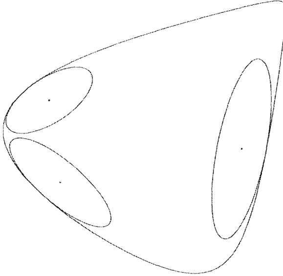
Figure 6.2. A 2D cross section of S^3_+ and cross sections of three Dikin ellipsoids.
