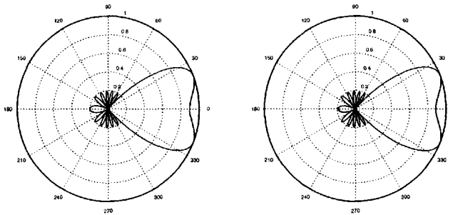
Figure 4.24. Robust design, actual pattern functions. Left: perturbation level \epsilon = 0.005 , sidelobe attenuation level -14.07\text{dB} \approx 0.20 , actual ripple 0.97\text{dB} \approx 1.12 . Right: perturbation level \epsilon = 0.05 , sidelobe attenuation level -13.43\text{dB} \approx 0.21 , actual ripple 1.04\text{dB} \approx 1.13 .
