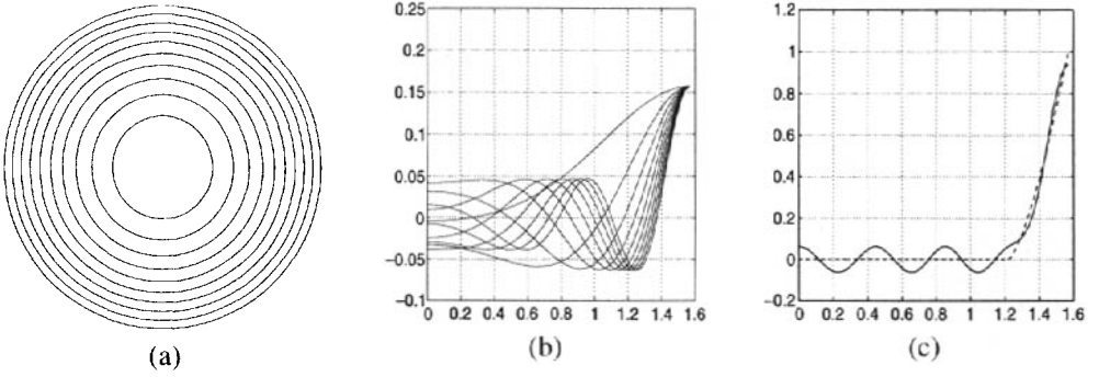
Figure 1.3. Synthesis of antennae array. (a): 10 array elements of equal areas in the XY -plane the outer radius of the largest ring is 1m, the wavelength is 50cm. (b): “building blocks” – the diagrams of the rings as functions of the altitude angle \theta . (c): the target diagram (dashed) and the synthesised diagram (solid).
