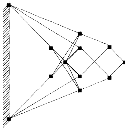
Figure 1.8. Ground structure and optimal truss (24 bars).
