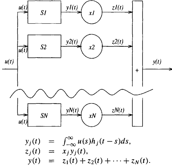
Figure 1.1. Parallel structure with amplifiers.
