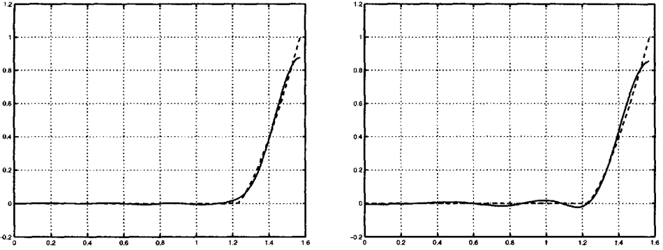
Figure 4.8. Dream and reality: the nominal least squares diagram (left, solid line) and an actual diagram yielded by robust least squares (right, solid line). Dashed lines are the target diagram.
