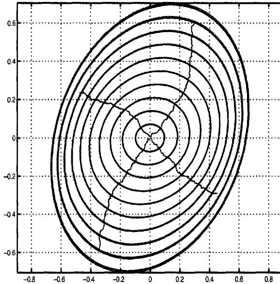
Figure 4.17. Outer and inner approximations of the reachability domains D^{10\ell} = D_{0,1\ell \text{ sec}} , \ell = 1, 2, \dots, 10 , for system (4.9.120). Ten pairs of ellipses are the outer and inner approximations of the domains D^1, \dots, D^{10} . (Look how close the ellipses from a pair are to each other!) Four curves are sample trajectories of the system. (Dots correspond to time instants 0.1\ell seconds in continuous time, i.e., time instants 10\ell in discrete time, \ell = 0, 1, \dots, 10 .)
