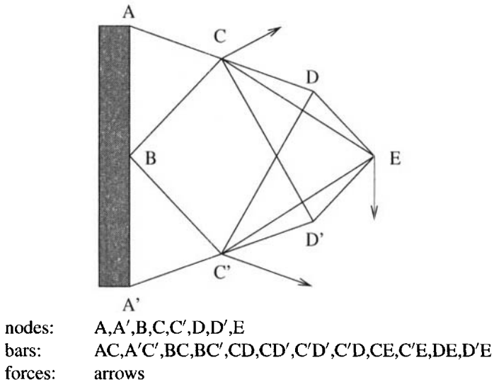
Figure 1.5. A simple planar truss and a load.
