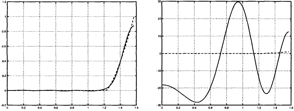
Figure 4.7. Dream and reality: the nominal diagram (left, solid line) and an actual diagram (right, solid line). Dashed lines are the target diagram. The target diagram varies from 0 to 1, and the nominal diagram (the one corresponding to x_j = x_j^* ) is at the \|\cdot\|_2 -distance 0.0178 from the target diagram. An actual diagram varies from \approx -30 to \approx 30 and is at the \|\cdot\|_2 -distance 20.0 (1124 times larger!) from the target.
