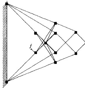
Figure 4.15. Optimal cantilever (single-load design); the compliance is 1.000.
