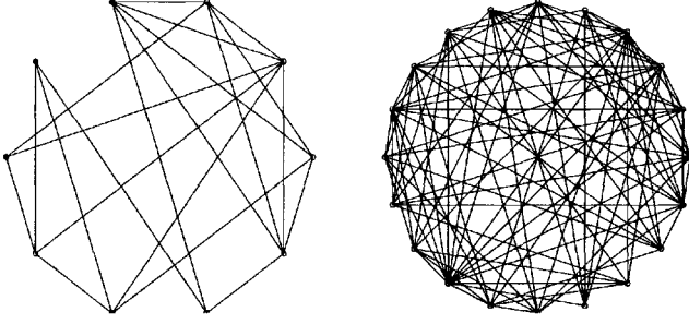
Figure 4.18. Graphs 13 (left) and 8 (right); all nodes are on circumferences.
