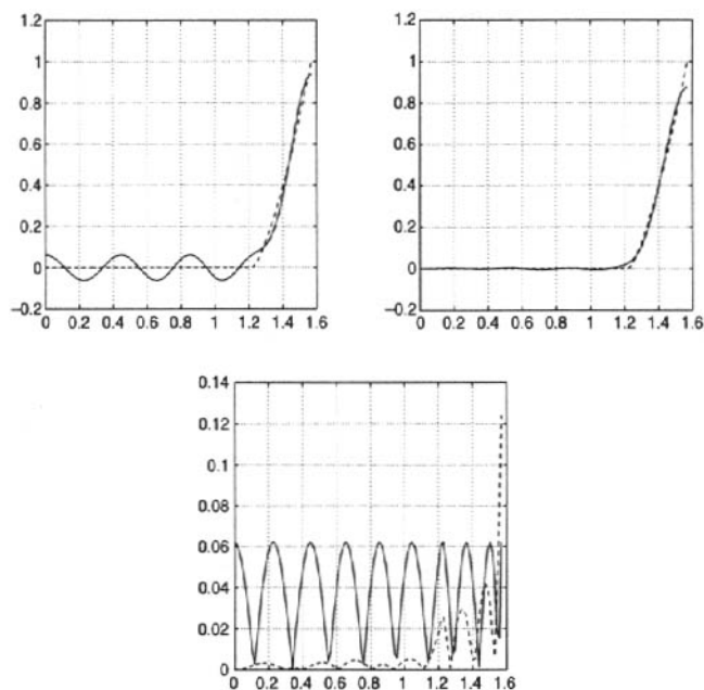
Figure 1.4. Top: Best uniform approximation (left) versus the least squares approximation (right). Bottom: Errors of the least squares (dashed) and the best uniform (solid) approximations.
