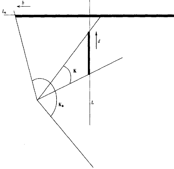
Figure 2.1. Primal-dual pair of conic problems. Bold lines: primal (vertical segment) and dual (horizontal ray) feasible sets.
