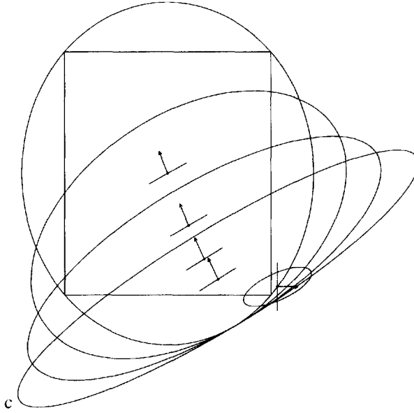
Figure 5.2. Ellipses E_{t-1} and search points c_{t-1} , t = 1, 2, 3, 4, 16 . Arrows: gradients of the objective f(x) ; unmarked segments: tangents to the level lines of f(x) .
