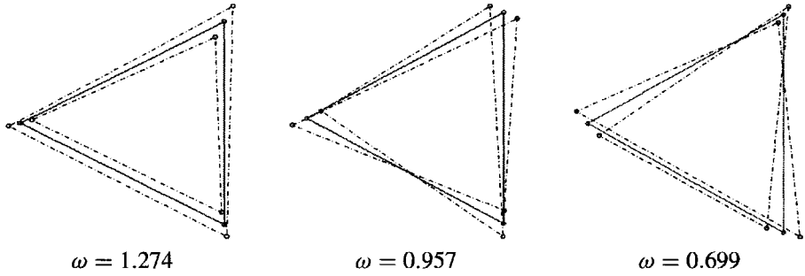
Figure 4.5. Nontrivial modes of a spring triangle (three unit masses linked by springs). Shown are three eigenmotions (modes) of a spring triangle with nonzero frequencies. Three instant positions of the oscillating triangle are depicted. There are three more eigenmotions with zero frequency, corresponding to shifts and rotation of the triangle.
