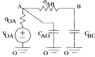
Figure 4.10. A simple circuit. Element OA: outer supply of voltage V_{OA} and resistor with conductance \sigma_{OA} . Element AO: capacitor with capacitance C_{AO} . Element AB: resistor with conductance \sigma_{AB} . Element BO: capacitor with capacitance C_{BO} .
