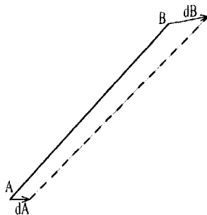
Figure 1.6. A bar before (solid) and after (dashed) load is applied.
