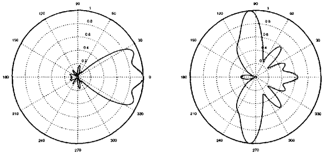
Figure 4.23. The reality. Left: perturbation level \epsilon = 0.005 , sidelobe attenuation level -15.12\text{dB} \approx 0.18 , actual ripple 1.65\text{dB} \approx 1.21 . Right: perturbation level \epsilon = 0.025 , sidelobe attenuation level 3.89\text{dB} \approx 1.56 , actual ripple 4.45\text{dB} \approx 1.67 .
