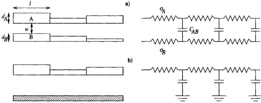
Figure 4.12. Wires (left) and the equivalent RC-structure (right). (a) a pair of two neighboring wires; (b) a wire and the substrate.
