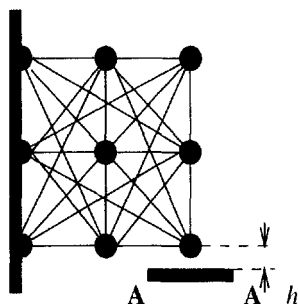
Figure 4.13. An obstacle. What we see is a nine-node planar ground structure with 33 tentative bars and a rigid obstacle AA. This obstacle does not allow the southeastern node to move down more than by h and thus induces a linear inequality constraint on the vector of virtual displacements of the nodes.
