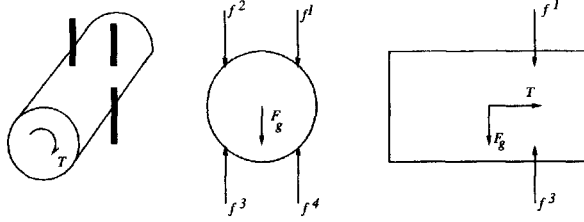
Figure 3.2. Perspective, front and side views.
