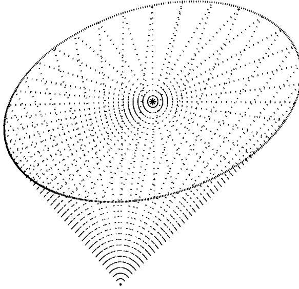
Figure 6.3. Conic cap of L^3 associated with X = \begin{pmatrix} 0.3 \\ 0 \\ 1 \end{pmatrix} .
