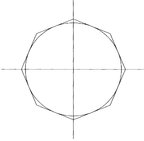
Figure 1.2. The contours |z| = 1 (circle) and p_4(z) = 1 (polygon).
