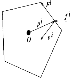
Figure 3.1. Geometry of i th contact. p^i is the contact point; f^i is the contact force; v^i is the inward normal to the surface.
