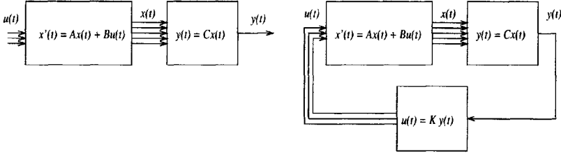
Figure 4.6. Open-loop (left) and closed-loop (right) controlled systems.
