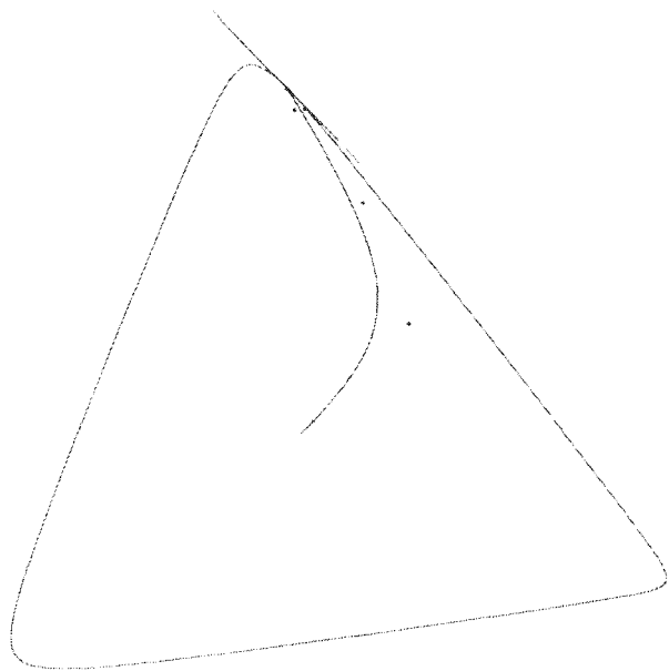
Figure 6.1. Primal path-following method. What you see is the 2D feasible set of a toy SDP ( \mathbf{K} = \mathbf{S}^3_+ ). The continuous curve is the primal central path; dots are iterates x_i of the algorithm. We cannot draw the dual solutions, since they live in four-dimensional space ( \dim \mathcal{L}^\perp = \dim \mathbf{S}^3 - \dim \mathcal{L} = 6 - 2 = 4 ).
