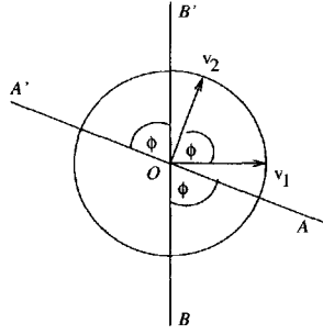
Figure 4.3. Computing the expected weight of random cut. w is the projection of v on the 2D plane spanned by v_1 and v_2 . The direction of w is uniformly distributed in [0, 2\pi] , and v separates v_1 and v_2 exactly when w belongs to one of the angles AOB, A'OB' .
