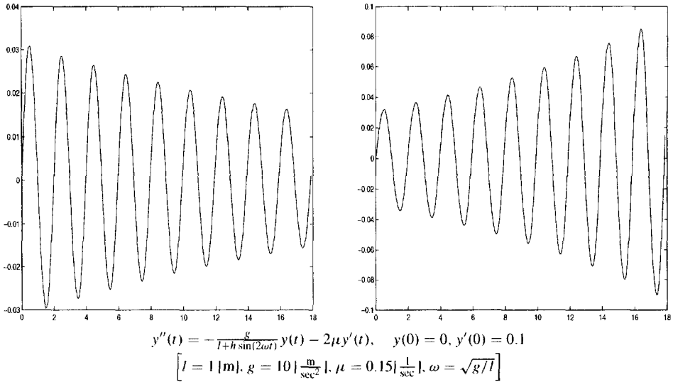
Figure 4.20. Graph of y(t) . Left: h = 0.125 ; this child is too small; he should grow up. Right: h = 0.25 ; this child can already swing.
