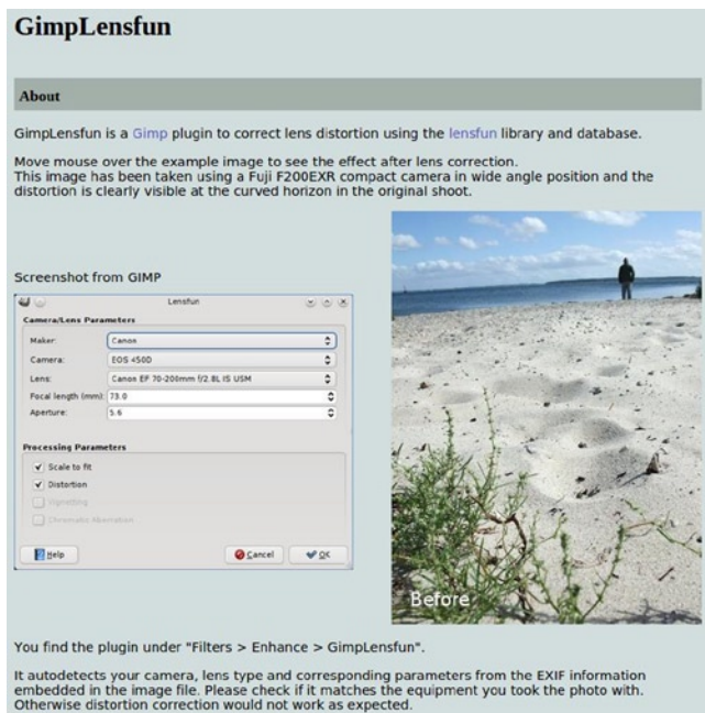
Figure 11. GimpLensFun is a useful plug-in for correcting lens distortion
