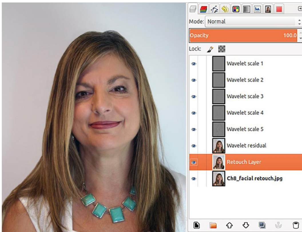
Figure 8-7. Wavelet scales
