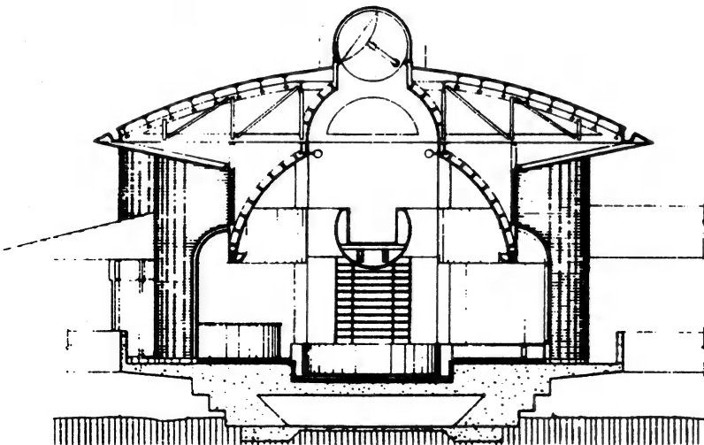
Cross section of energy self-sufficient home.
