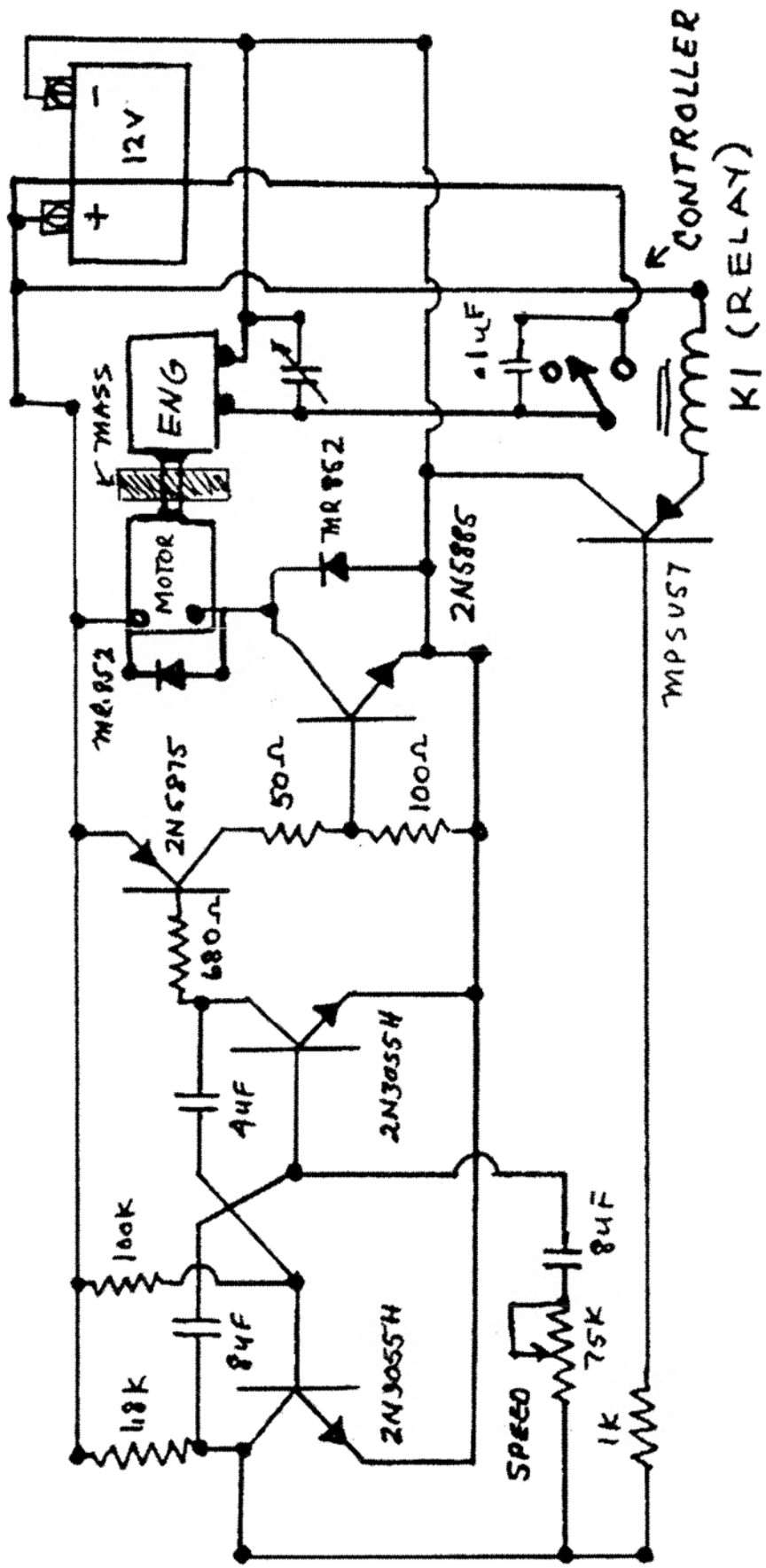
FIGURE 3. CIRCUIT FOR THE BEDINI FREE ENERGY DEVICE
