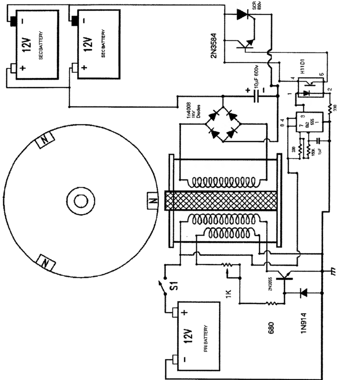
FIGURE 34. RADIANT ENERGY POWERING OF THE MONOPOLE MOTOR
