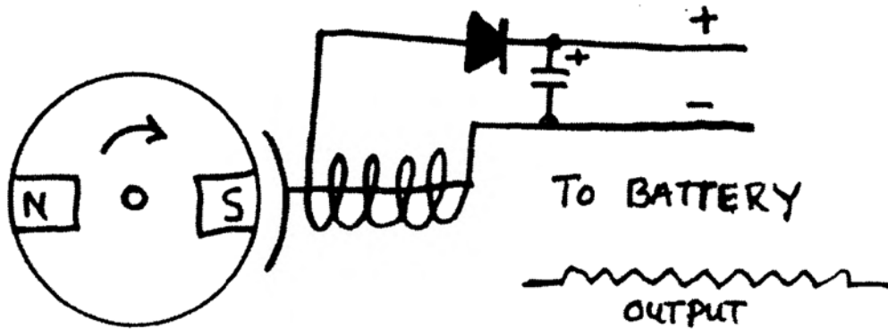
FIGURE 11. CONVENTIONAL EXPLANATION
