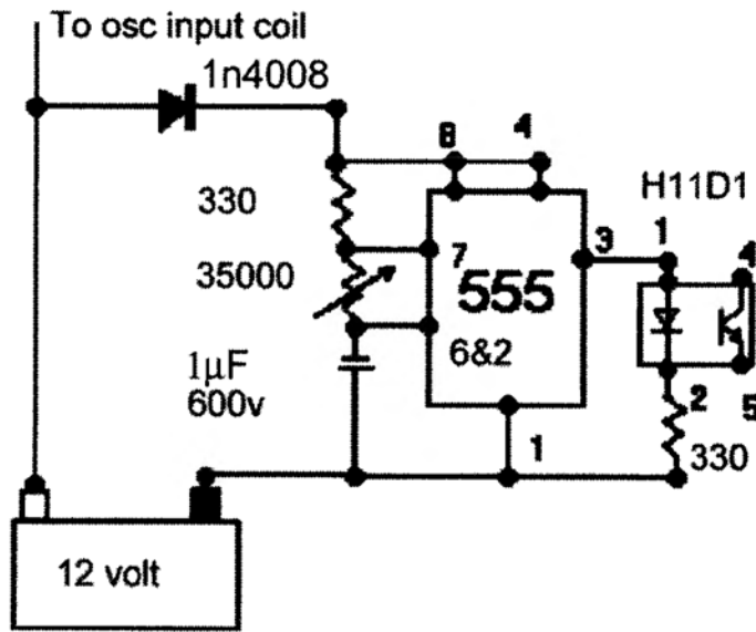
FIGURE 28 FREE RUNNING 555 TIMING CIRCUIT
