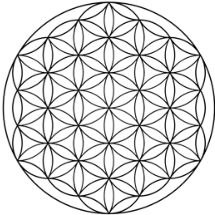
THE TERRYEN WAVE FIELDS
