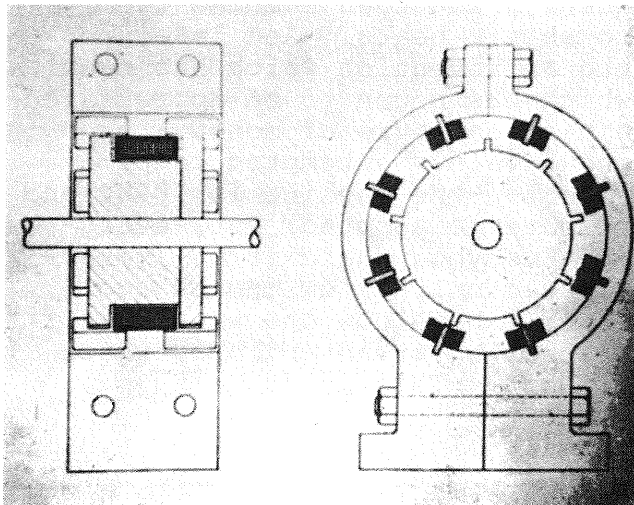
Figure 11. Another small high-frequency alternator of different construction intended for the same purposes. Drawing. Mercury interrupters, 1898.
