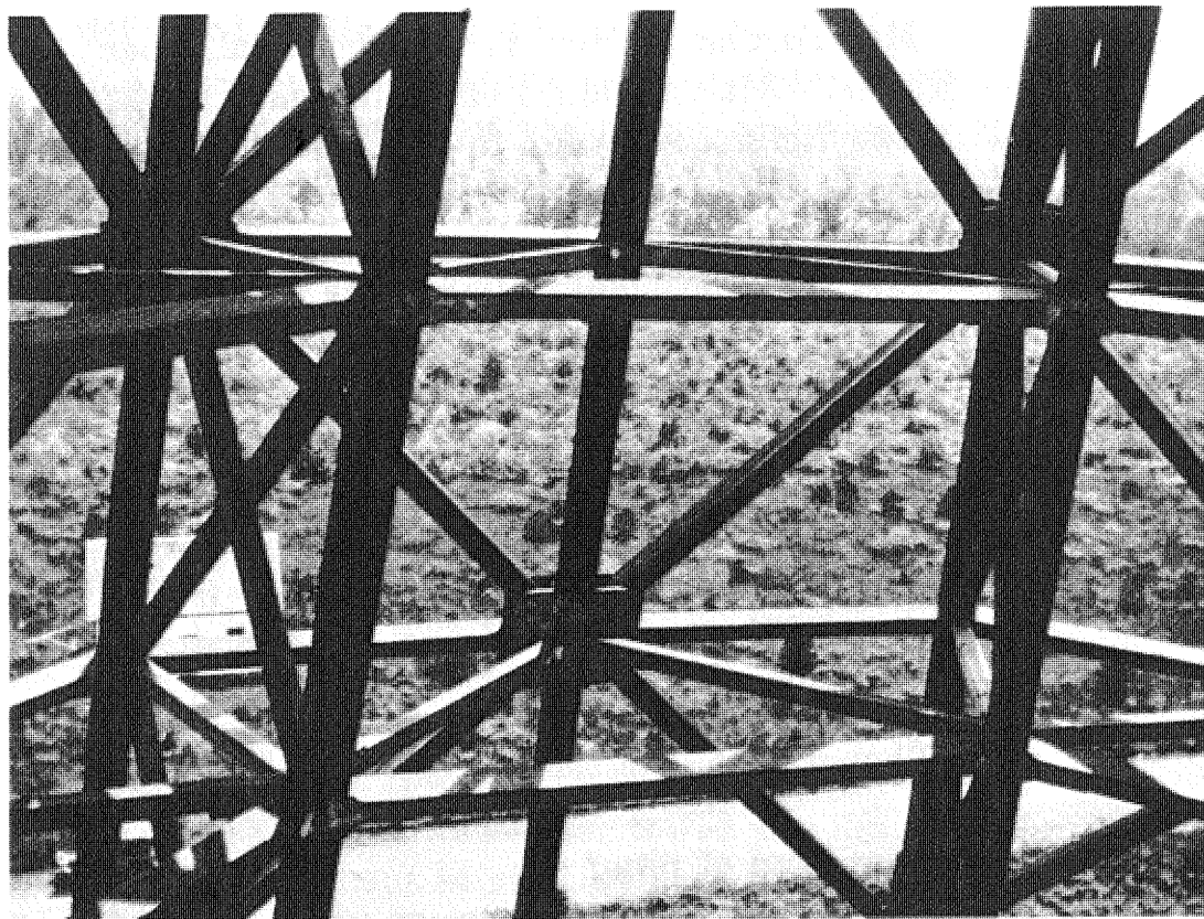
Figure A2-1 Construction detail of Wardencllyffe plant tower.
