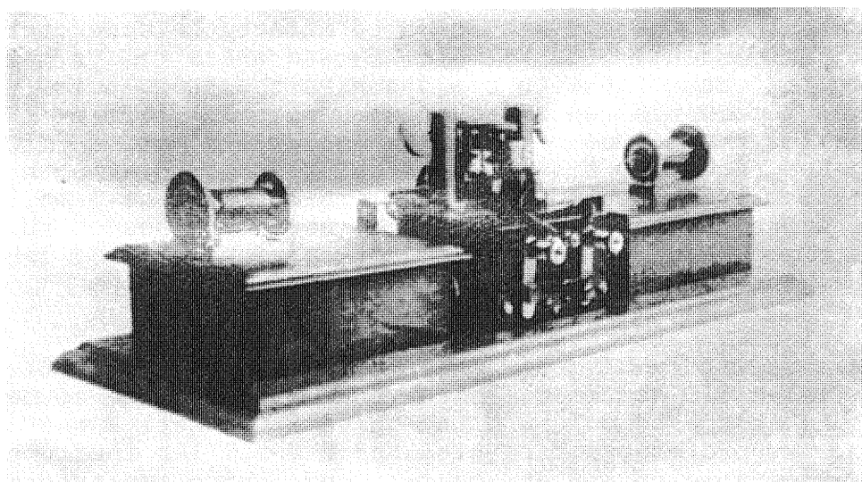
Figure 13. Instrument to receive radio waves of 1896-1899 structure.
