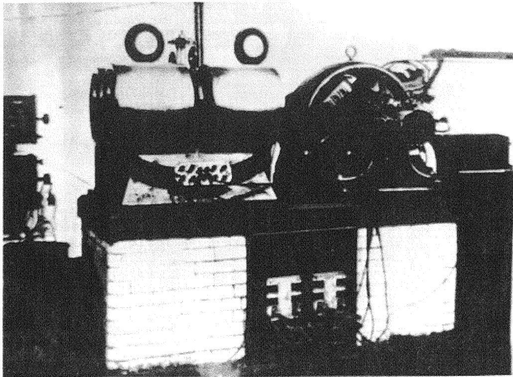
Figure 27. Large mechanical and electrical oscillator with four vibrating parts installed in the laboratory at 46 E. Houston Street, for furnishing isochronous currents of desired wave frequencies, phases, and beats.
