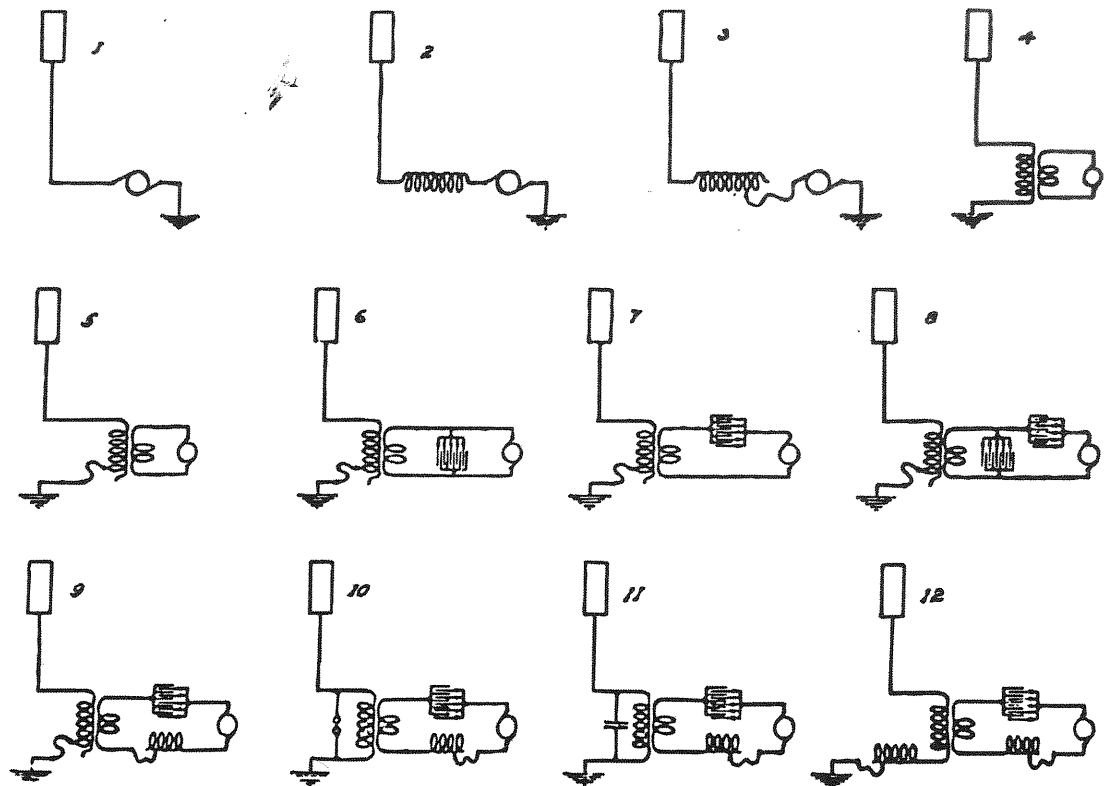
Figure 5. Illustrating various ways of using a high frequency alternator in the first experiments at the Grand Street Laboratory: 1891-1893.
