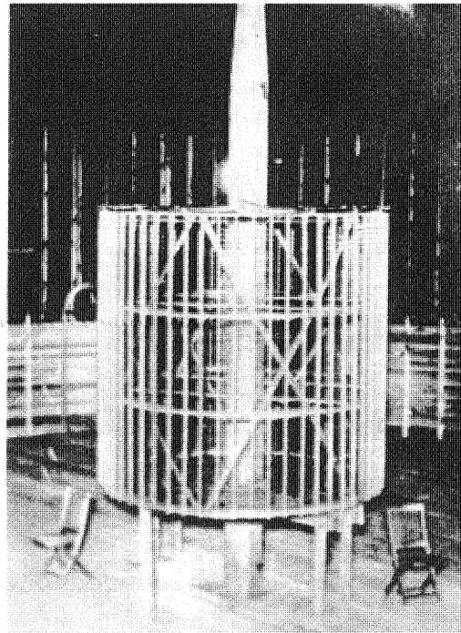
Figure 56. Illustrating another experiment with the same apparatus in which the coil is not directly connected to the source of oscillations, but receives the effect inductively from a distance. [Note: the wire lead used to connect the resonator to the ground plate is absent.]
