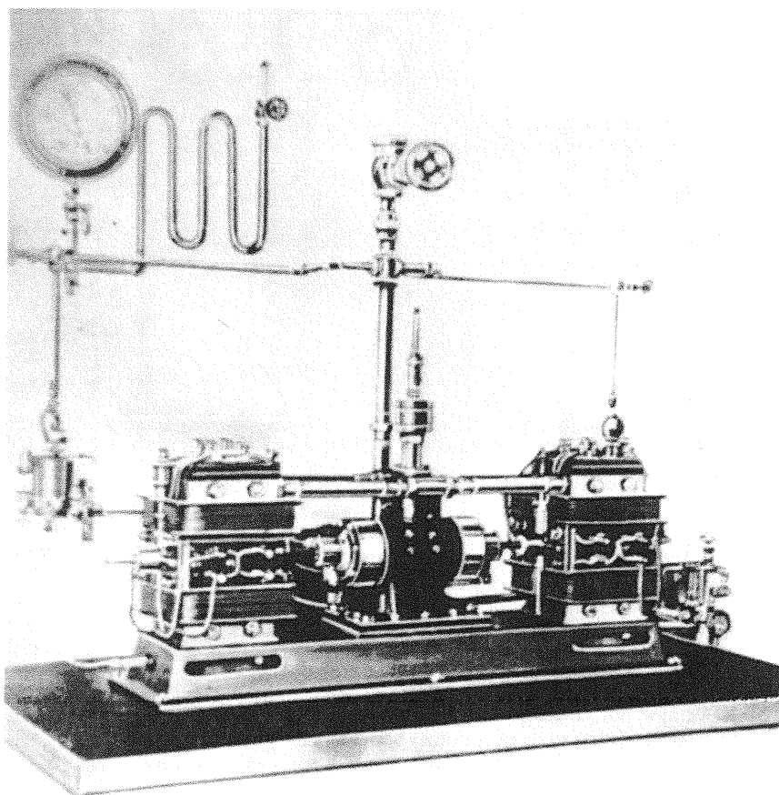
Figure 25. Double compound mechanical and electrical oscillator for generating current of perfect, constant, dynamo frequency of 10 horsepower. (Article by Martin ["Tesla's Oscillator and Other Inventions"], Century Magazine , April 1895, Fig. 2, p. 921.) (Built in 1893.)
