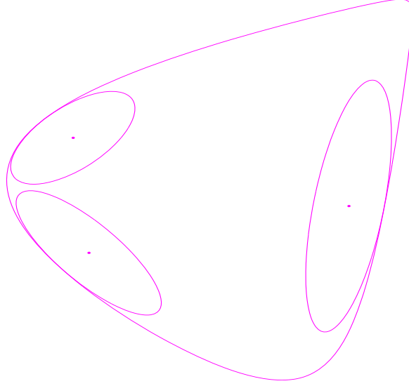
A 2D cross-section of \mathbf{S}_+^3 and cross-sections of 3 Dikin ellipsoids
