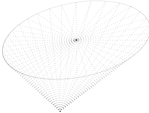
Figure 4.4: Conic cap of \mathbf{L}^3 associated with X = [0.3; 0; 1]
