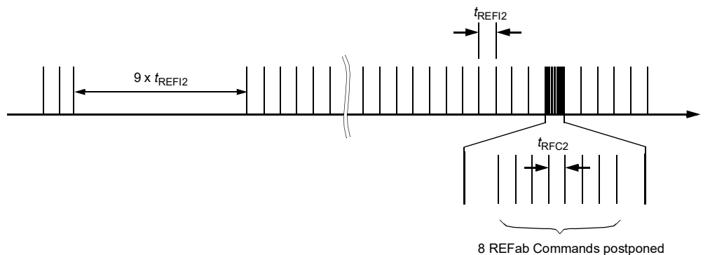
Figure 67 — Postponing Refresh Commands (Example of Fine Granularity Refresh Mode - t_{RFC2} )
