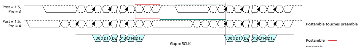
Figure 20 — Example of Consecutive Reads Operation: t_{CCD} = \text{Min} + 5
