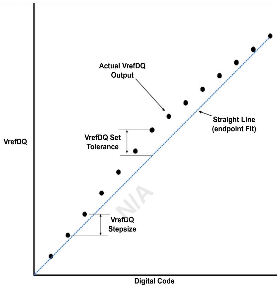
Figure 108 — Example of Vref Set Tolerance (Max Case Only Shown) and Stepsize
