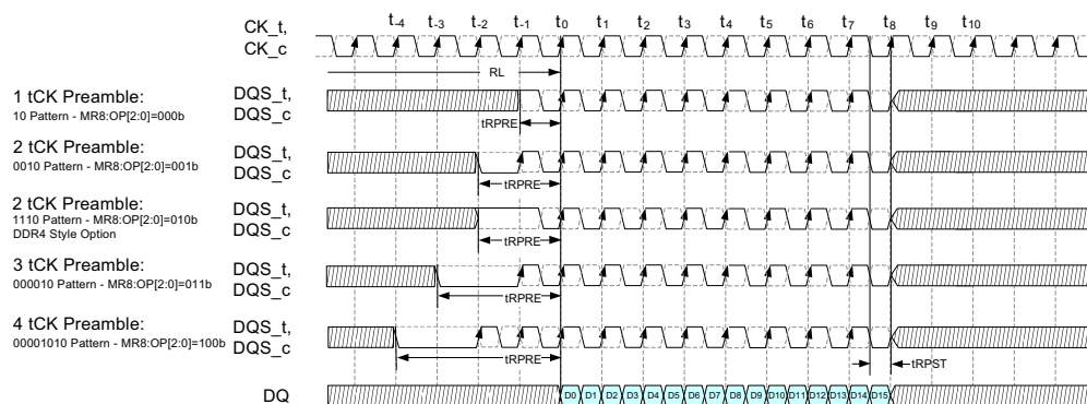
Figure 9 — Example of Read Preamble Modes (Default) w/0.5 tCK Postamble
