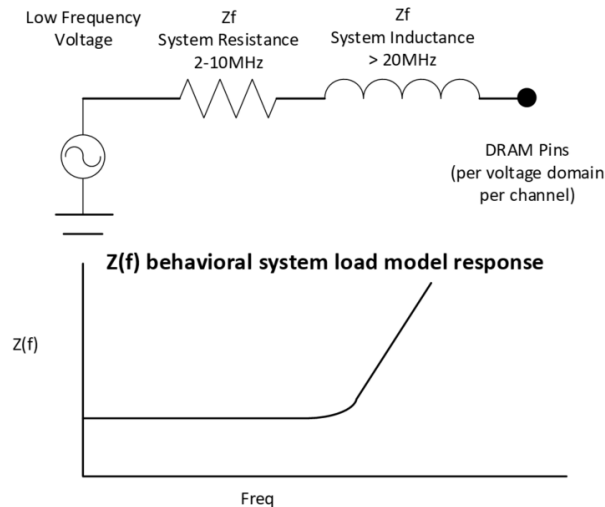
Figure 172 — Simplified Z(f) Electrical Model And Frequency Response of PDN at the DRAM Pin without the DRAM Component
