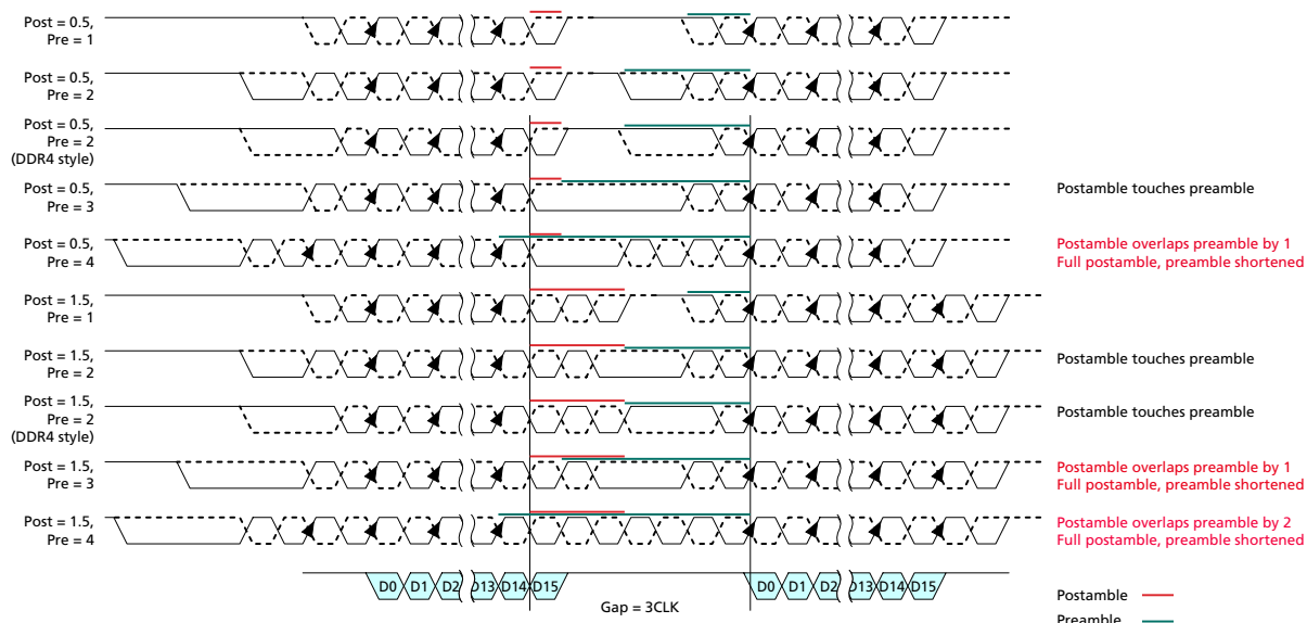
Figure 18 — Example of Consecutive Reads Operation: t_{CCD} = \text{Min} + 3
