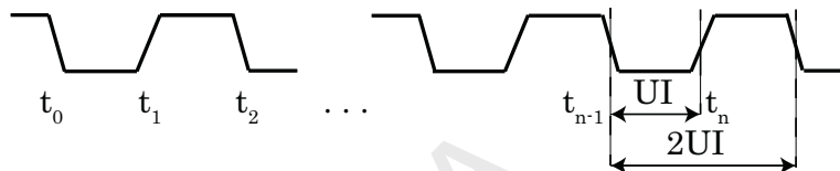
Figure 174 — UI Definition Using Clock Waveforms
