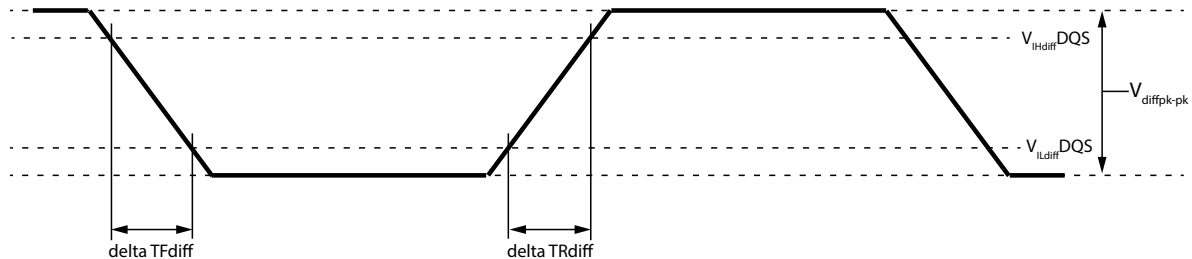
Figure 193 — Differential Input Slew Rate Definition for DQS t , DQS c
