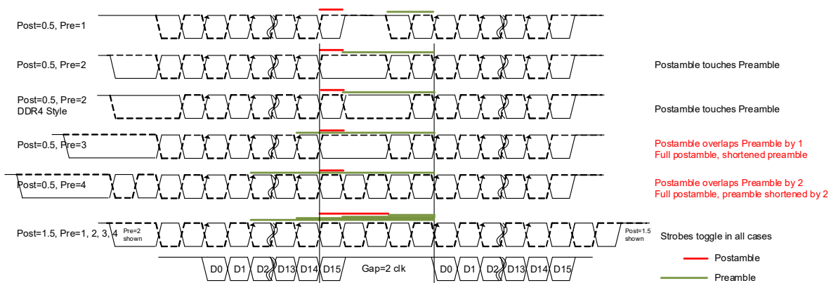
Figure 17 — Example of Consecutive Reads Operation: t CCD =Min+2
