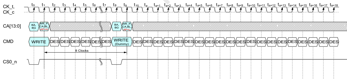
Figure 50 — Write with Auto-Precharge for Fixed BL32 and BL32 in BL32 OTF Mode
