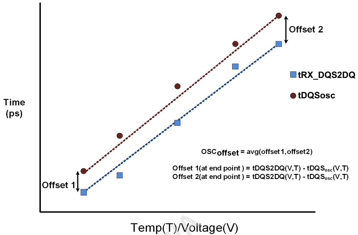
Figure 124 — Interval Oscillator Offset (OSC_offset)
