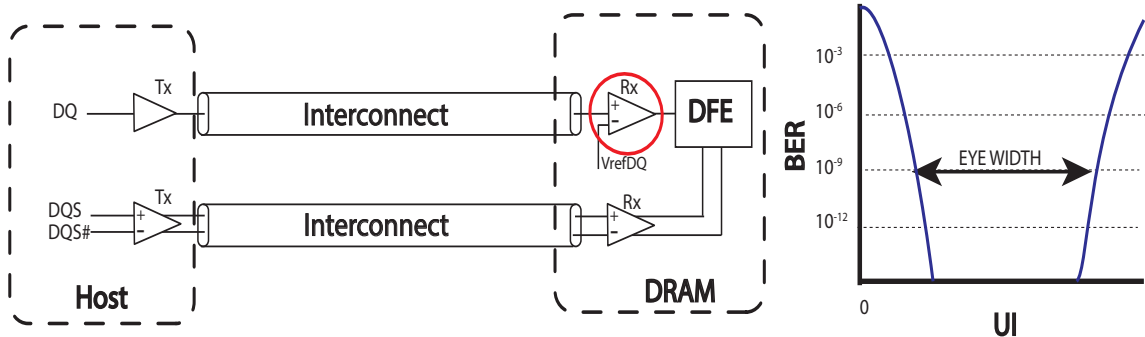
Figure 194 — Example of DDR5 Memory Interconnect
