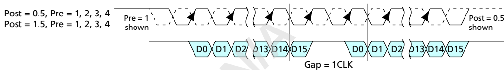
Figure 16 — Example of Consecutive Reads Operation: t CCD =Min+1
