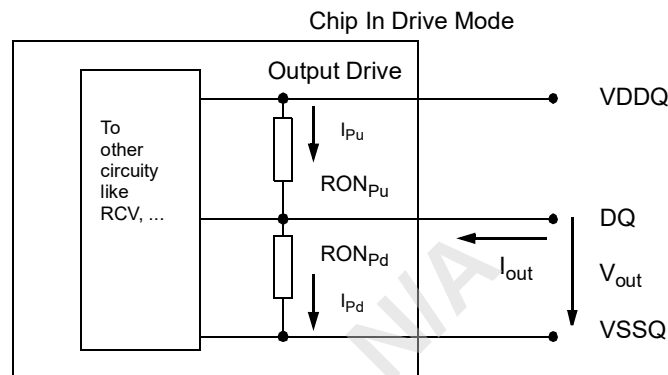
Figure 201 — Output Drive, Chip In Drive Mode
