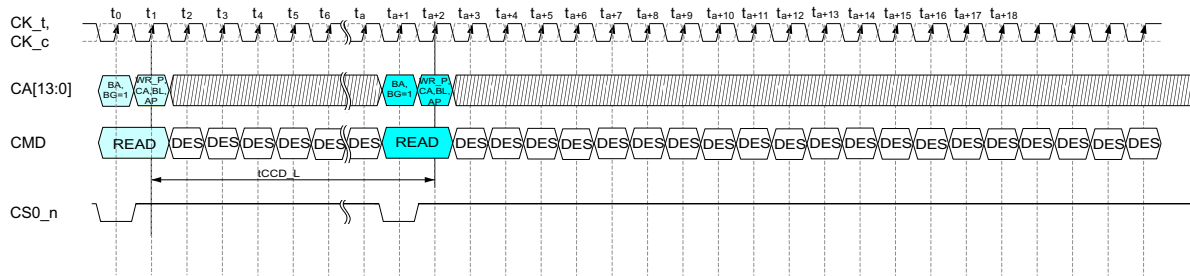
Figure 36 — Read to Read to Same Bank Group for BL16 in BL32 OTF
