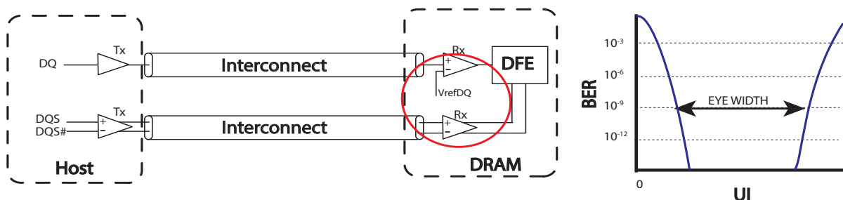
Figure 189 — SDRAM's Rx Forwarded Strokes for Jitter Sensitivity Testing
