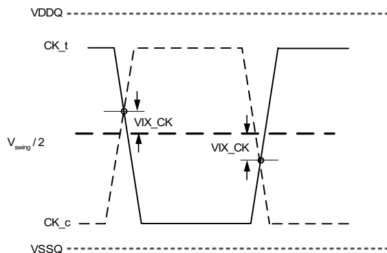
Figure 185 — VIX Definition (CK)
