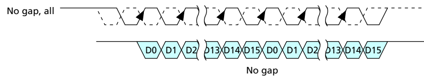
Figure 15 — Example of Seamless Reads Operation: t CCD =Min
