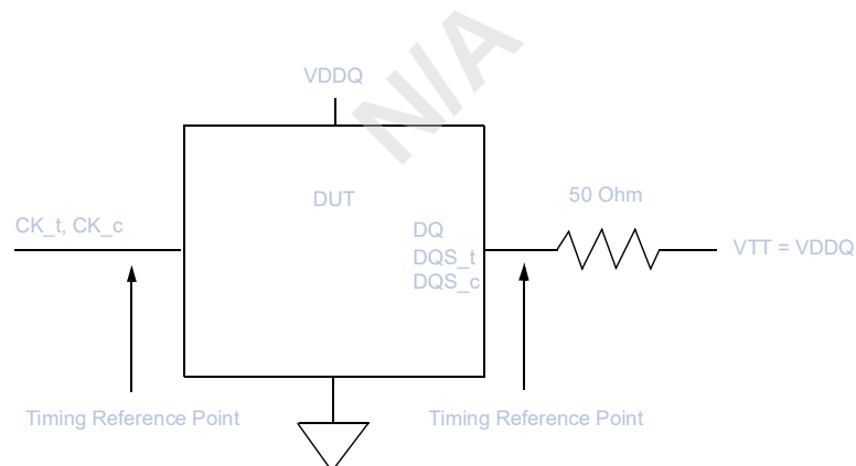
Figure 215 — Reference Load for AC Timing and Output Slew Rate
