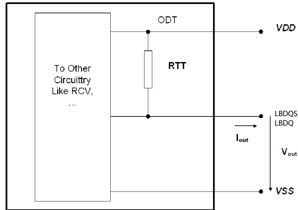
Figure 170 — Functional Representation of Loopback ODT
